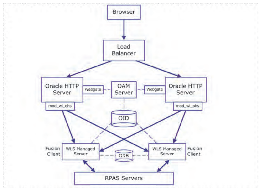
Figure 5-1 Load Balancer for a Non-SSO Deployment
