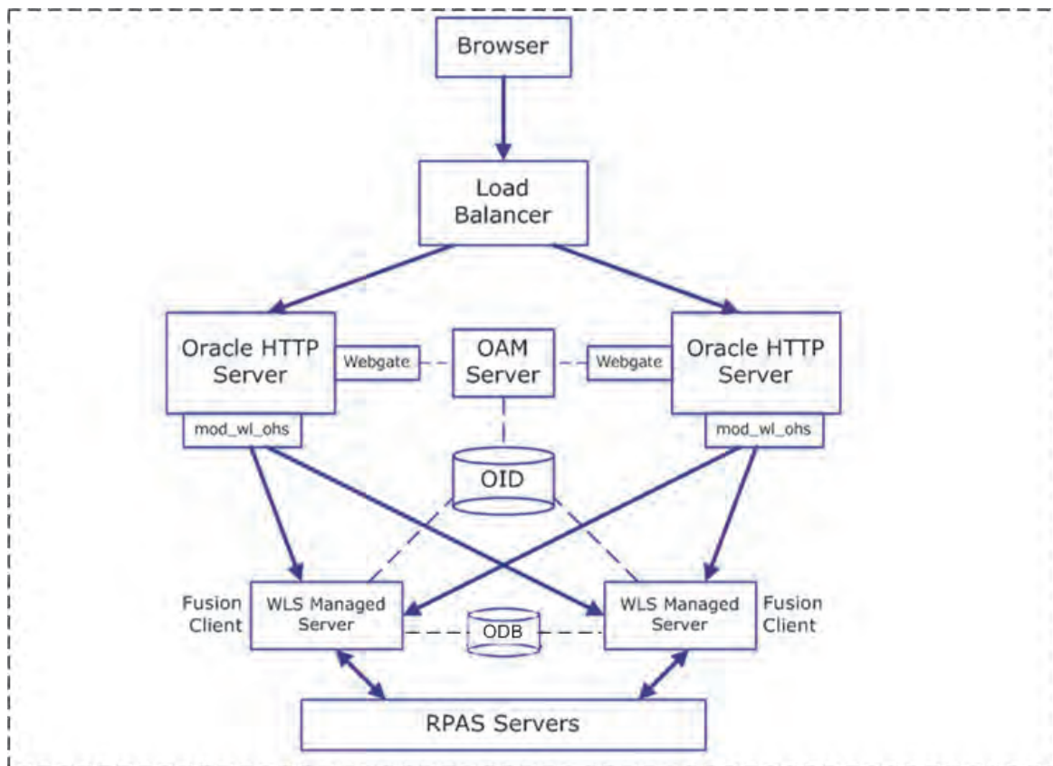
Figure 5–2 Load Balancer for an SSO Deployment
