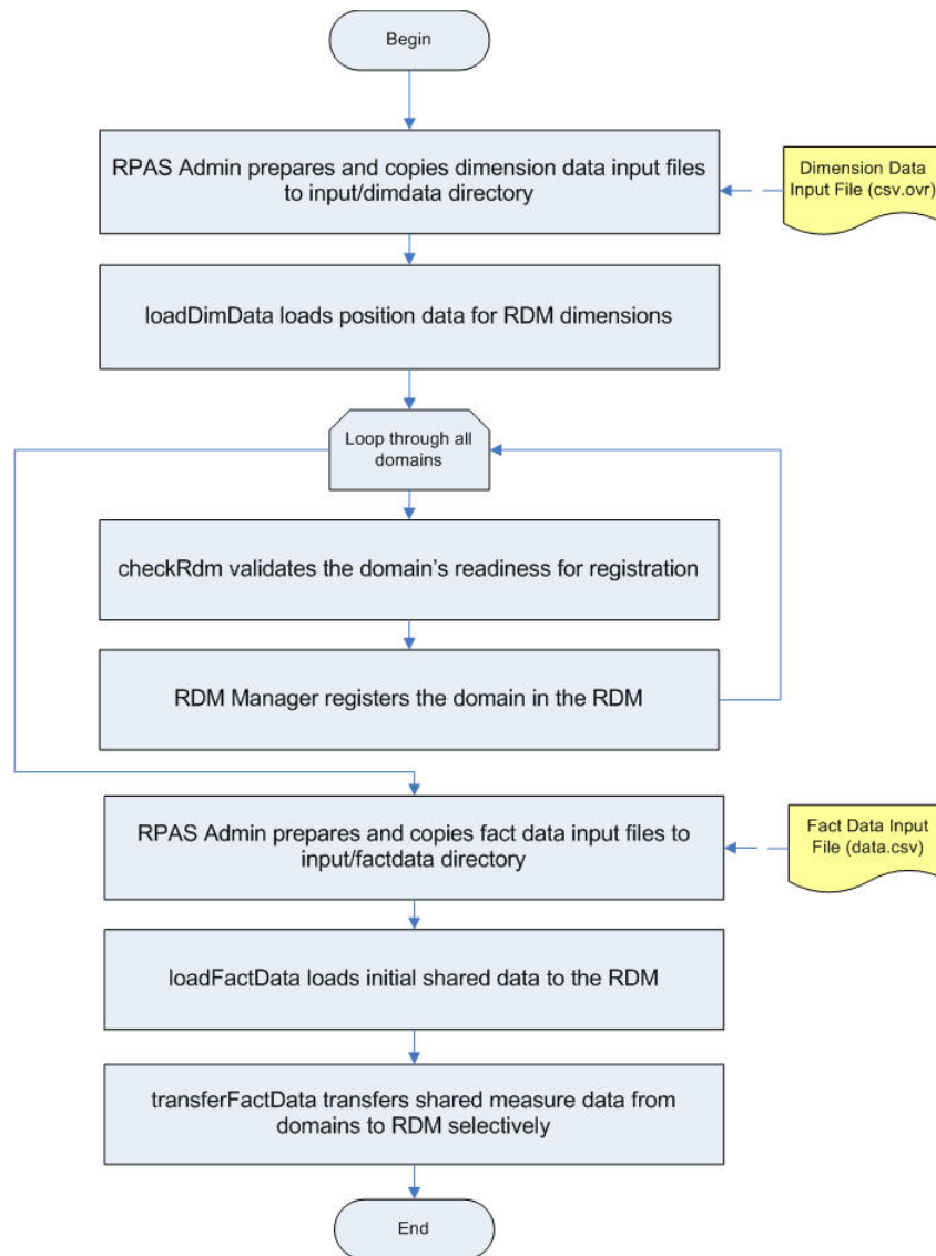
Figure 17-21 Post-Installation Steps
