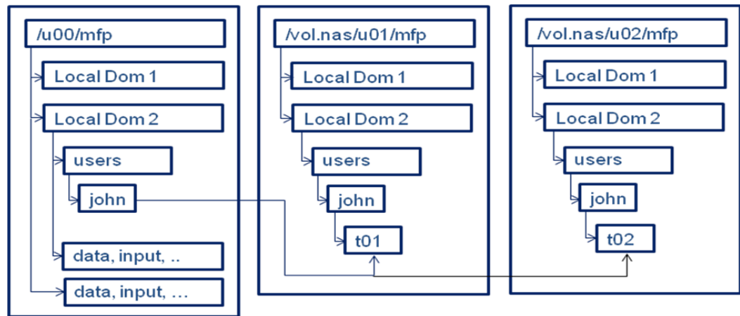
Example of Distributed Storage Directories
