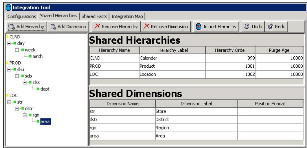
Shared Hierarchies Tab with the Selected Content Imported
