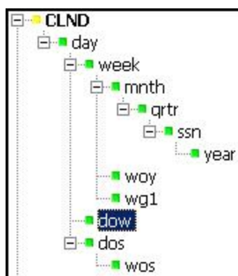
Example of Branch Hierarchy
