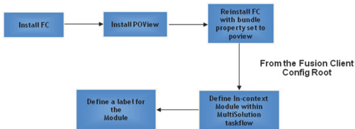
Figure E-2 Install and Configuration Sequence for POView
