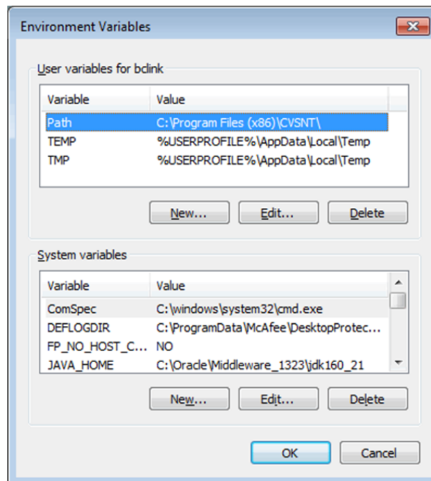
Figure 4–8 Environment Variables
