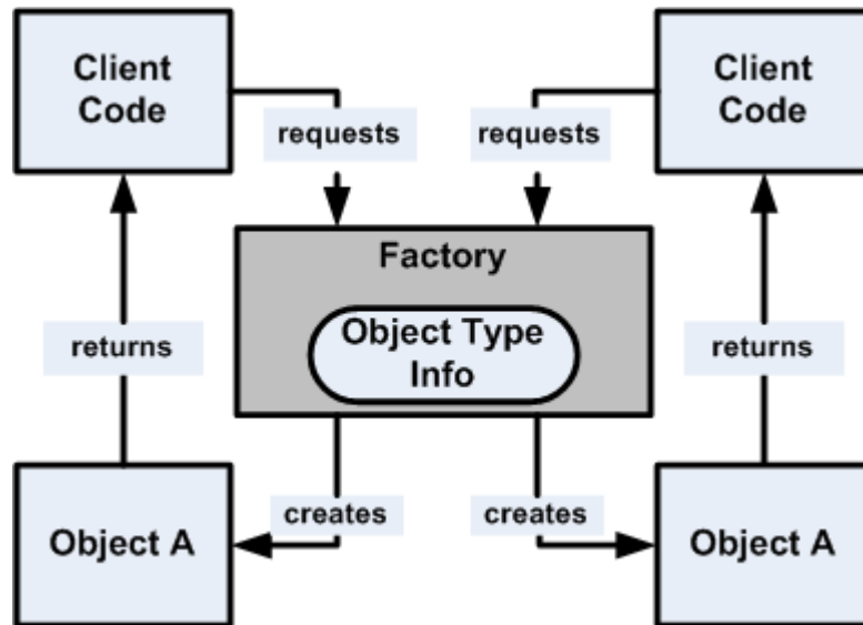
Figure 2–8 Factory Pattern
