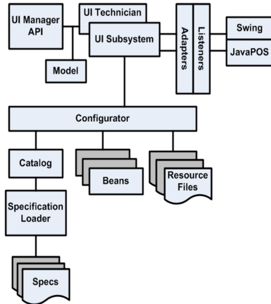
Figure 2-4 UI Framework
