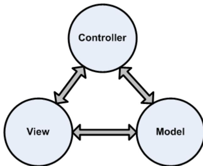
Figure 2–7 MVC Pattern
