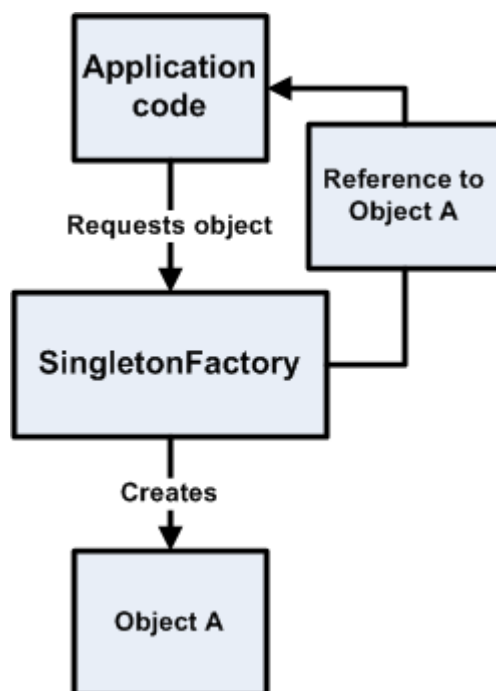
Figure 2–10 Singleton Pattern
