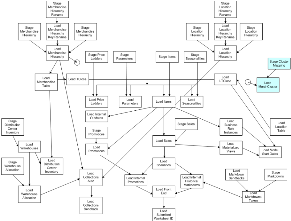
Figure 3–1 Dependency Tree
