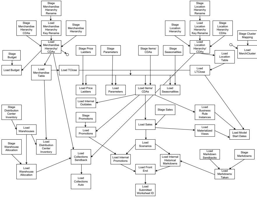
Figure 3–1 Standard Load Dependency Tree
