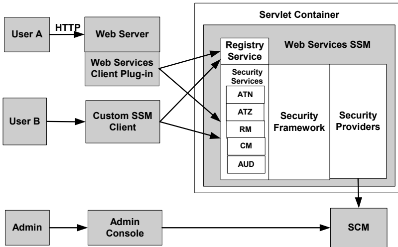
Figure 2-7 Usage Model
