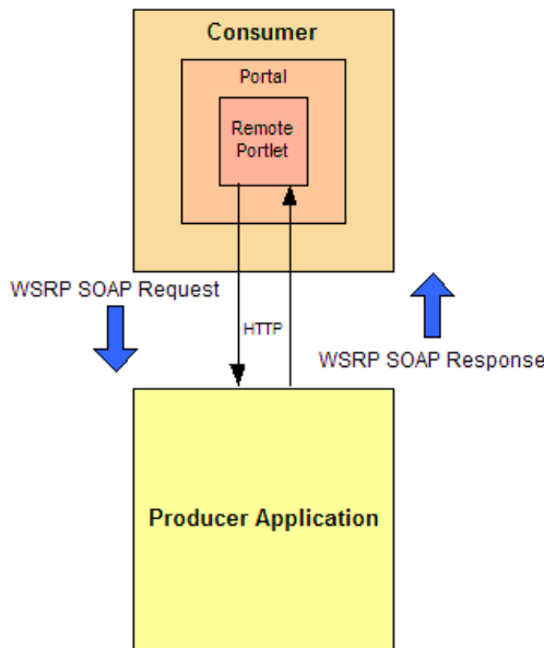
Figure 1-1 Basic Request/Response Flow Between Producer and Consumer Applications
