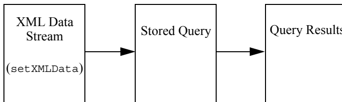
Figure 8-1 Setting XML Data as an input to a stored query
