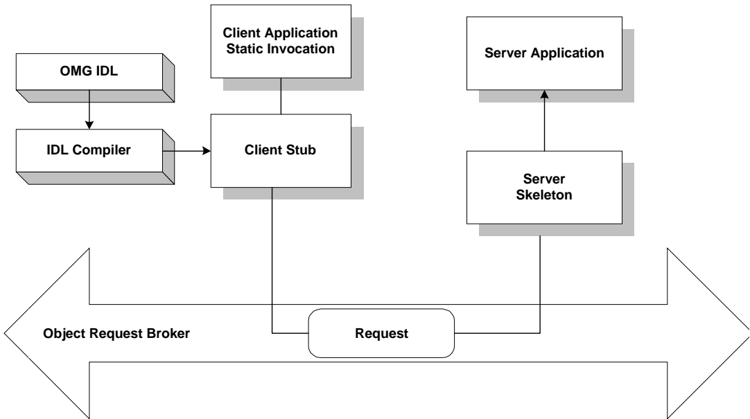
Figure 1-1 Static Invocation
