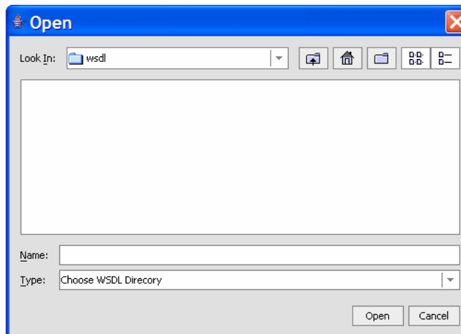
Figure 1-6 WSDL Location
