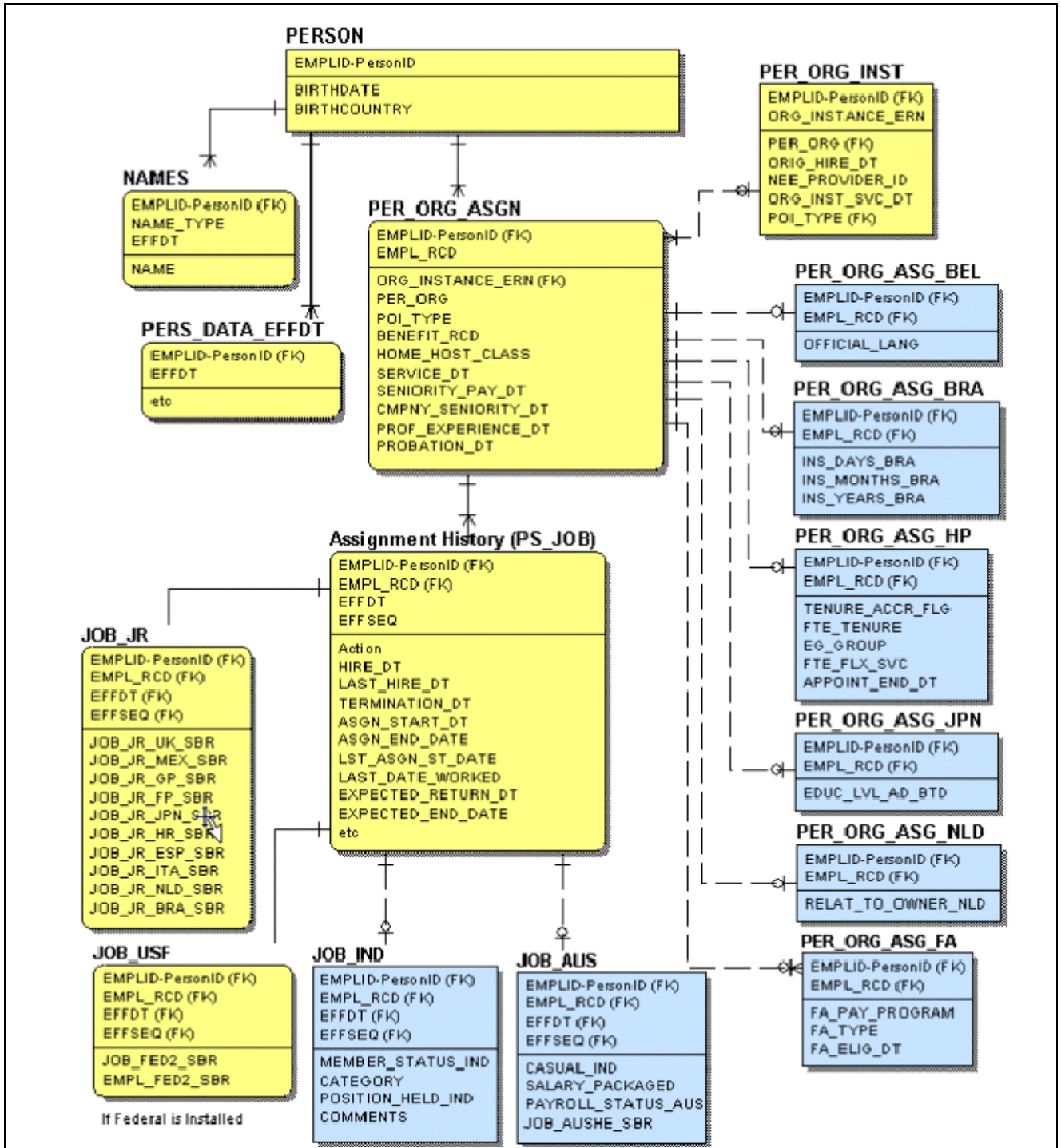
Worker ERD
