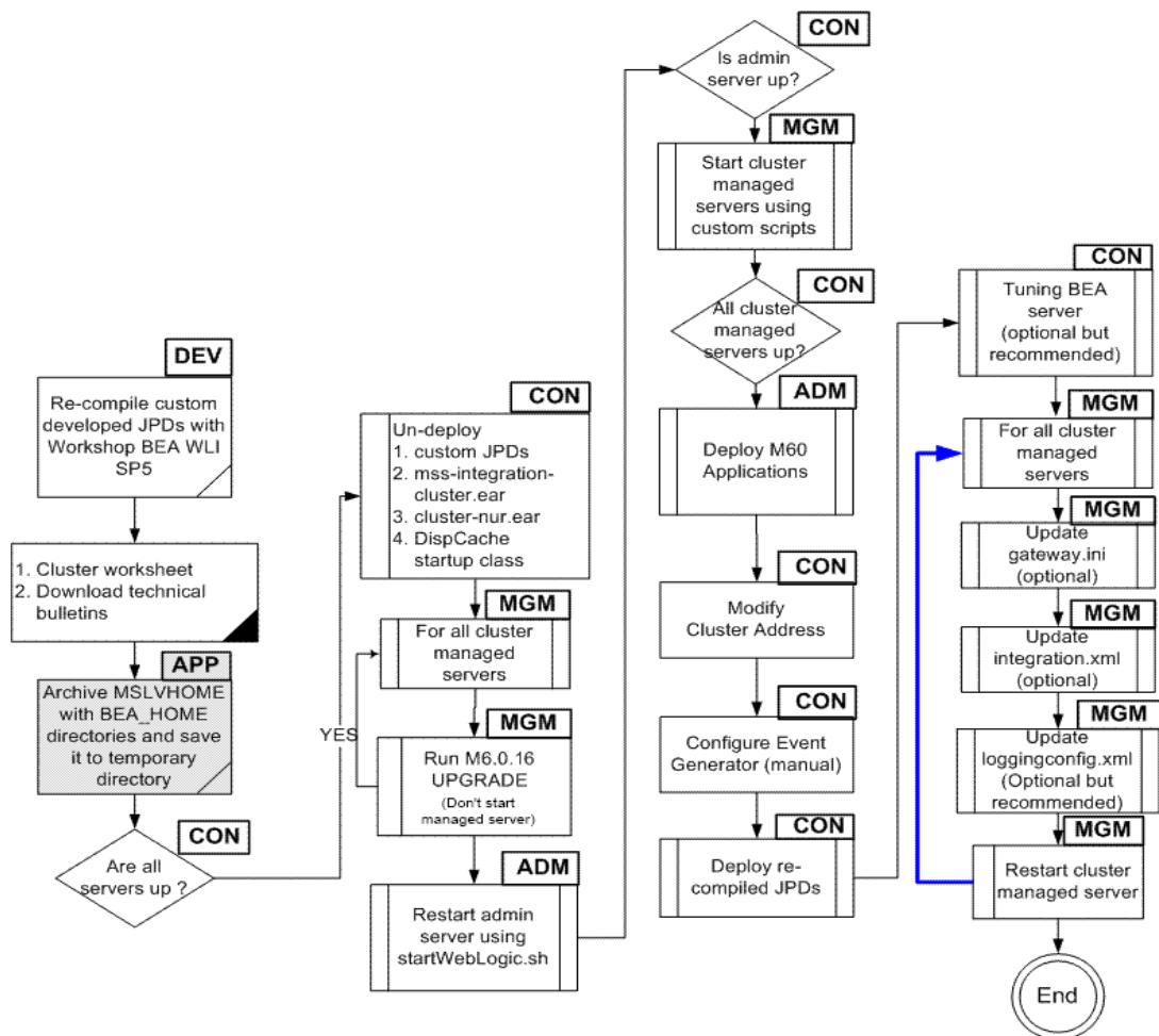
Figure 19: Upgrading a clustered configuration
