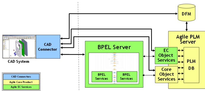
Abbildung 4: CAD integration architecture
