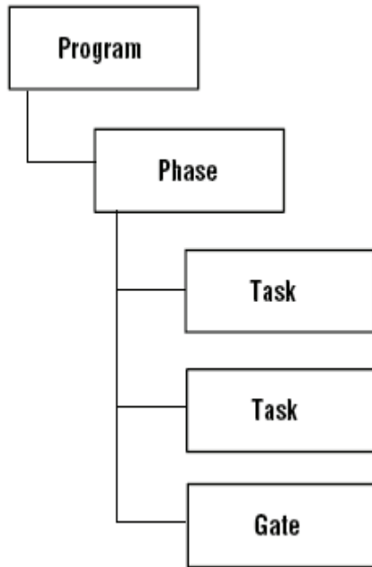
Figure 11: Program hierarchy
