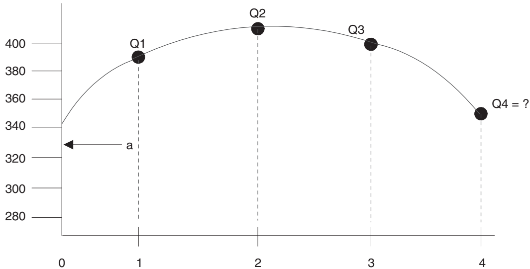
Figure 3–2 Plotting Q1, Q2, Q3, and Q4 for second degree approximation
