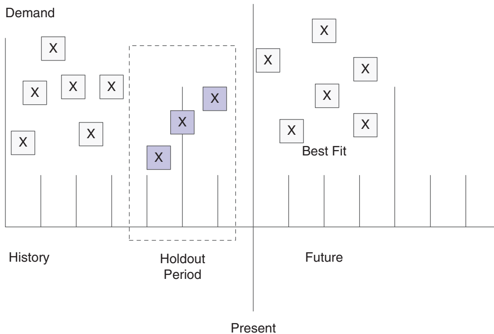
Figure 3–1 Best fit forecast
