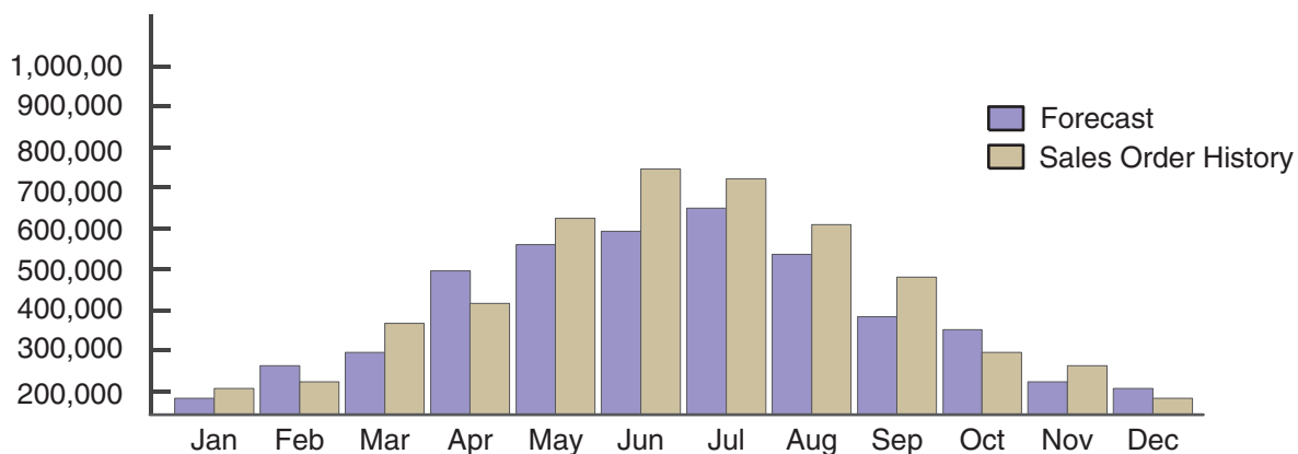
Figure 6–1 Comparing Forecast to Sales Order History
