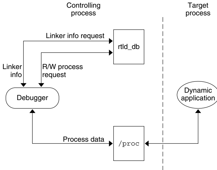
FIGURE 6-1 rtld-debugger Information Flow
