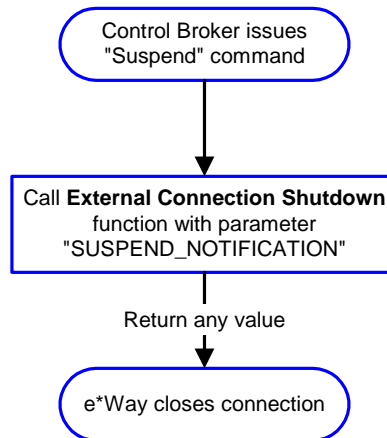
Figure 19 Disconnect Process
