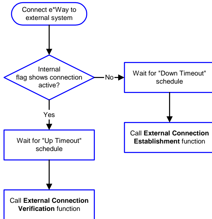
Figure 16 Connection Process
