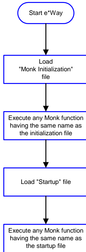
Figure 15 Initialization Process
