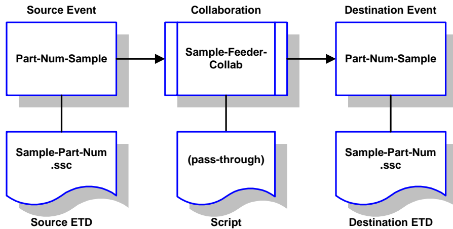
Figure 9 Sample-Feeder-Collab Collaboration
