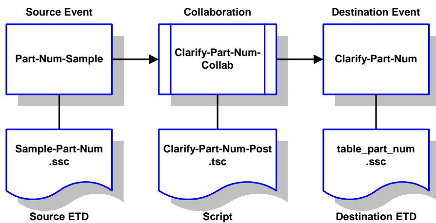
Figure 10 Clarify-Part-Num-Collab Collaboration
