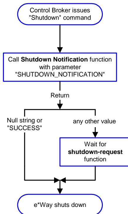
Figure 20 Shutdown Process
