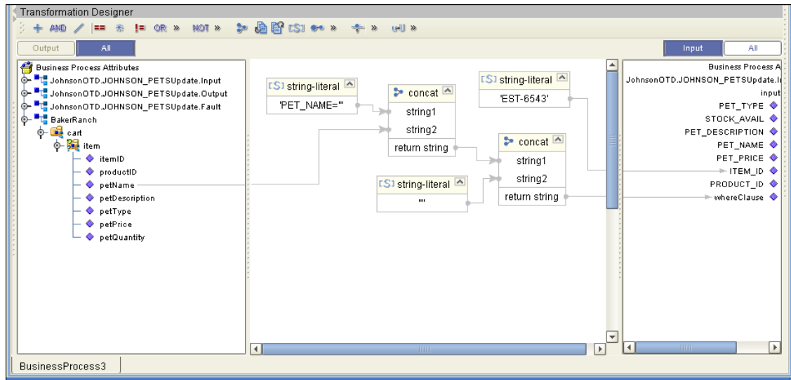
Figure 37 Update Input
