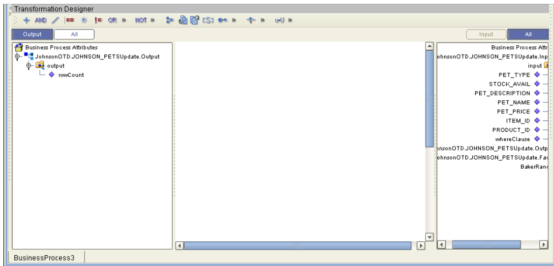
Figure 38 Update Output
