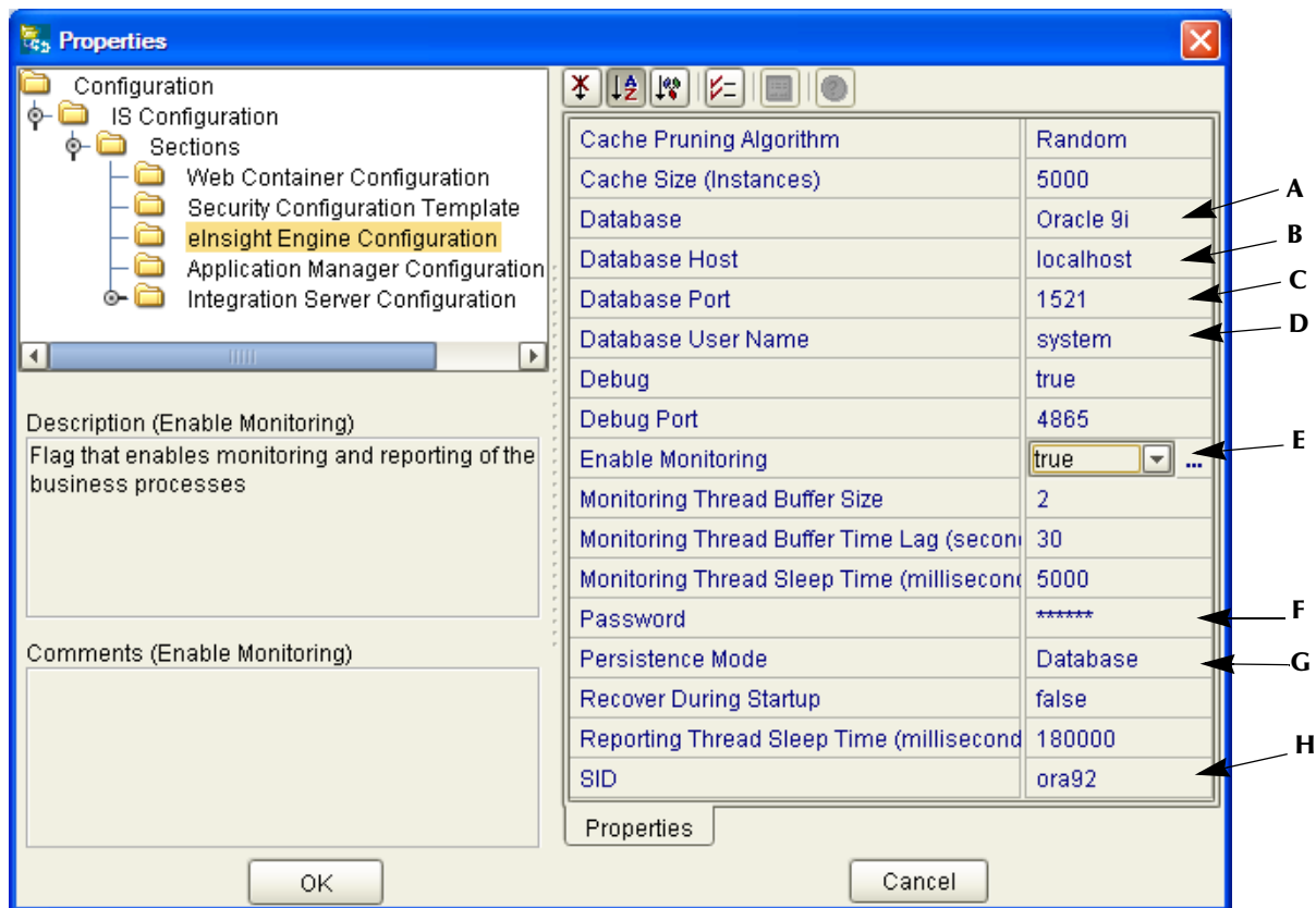
Figure 52 eInsight Engine Configuration
