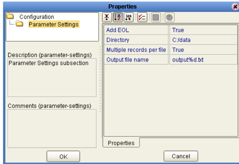
Figure 70 Outbound File eWay
