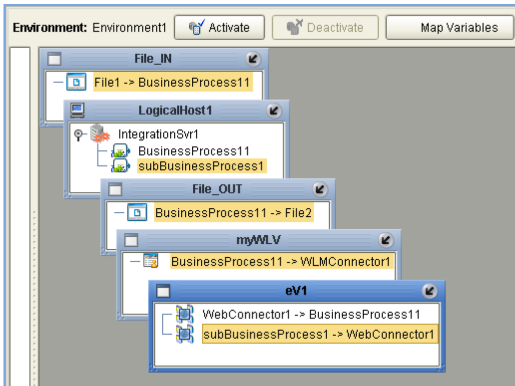
Figure 102 Worklist Manager Deployment Profile
