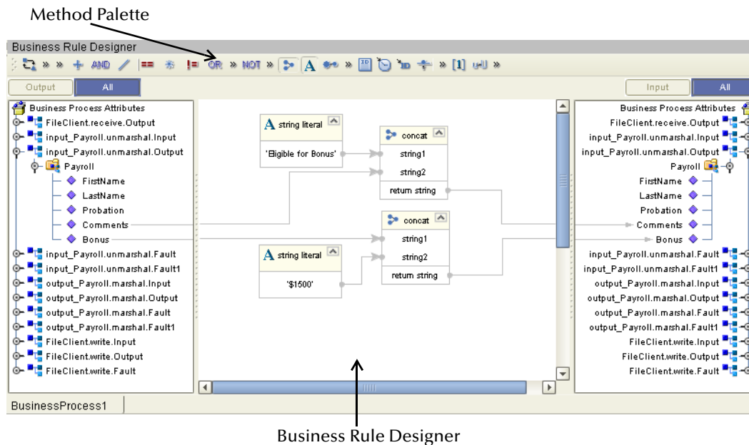
Figure 17 Business Rule Designer
