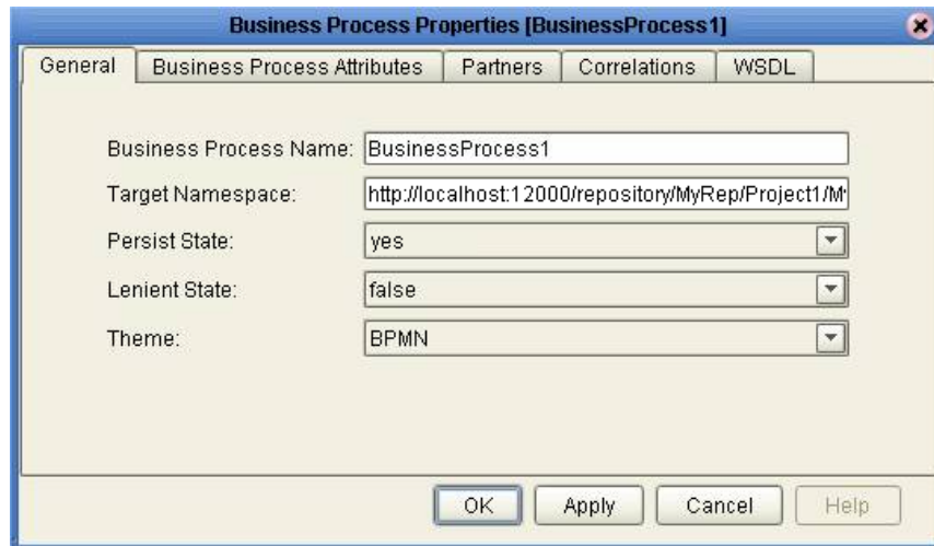
Figure 21 Business Process Properties: General Tab
