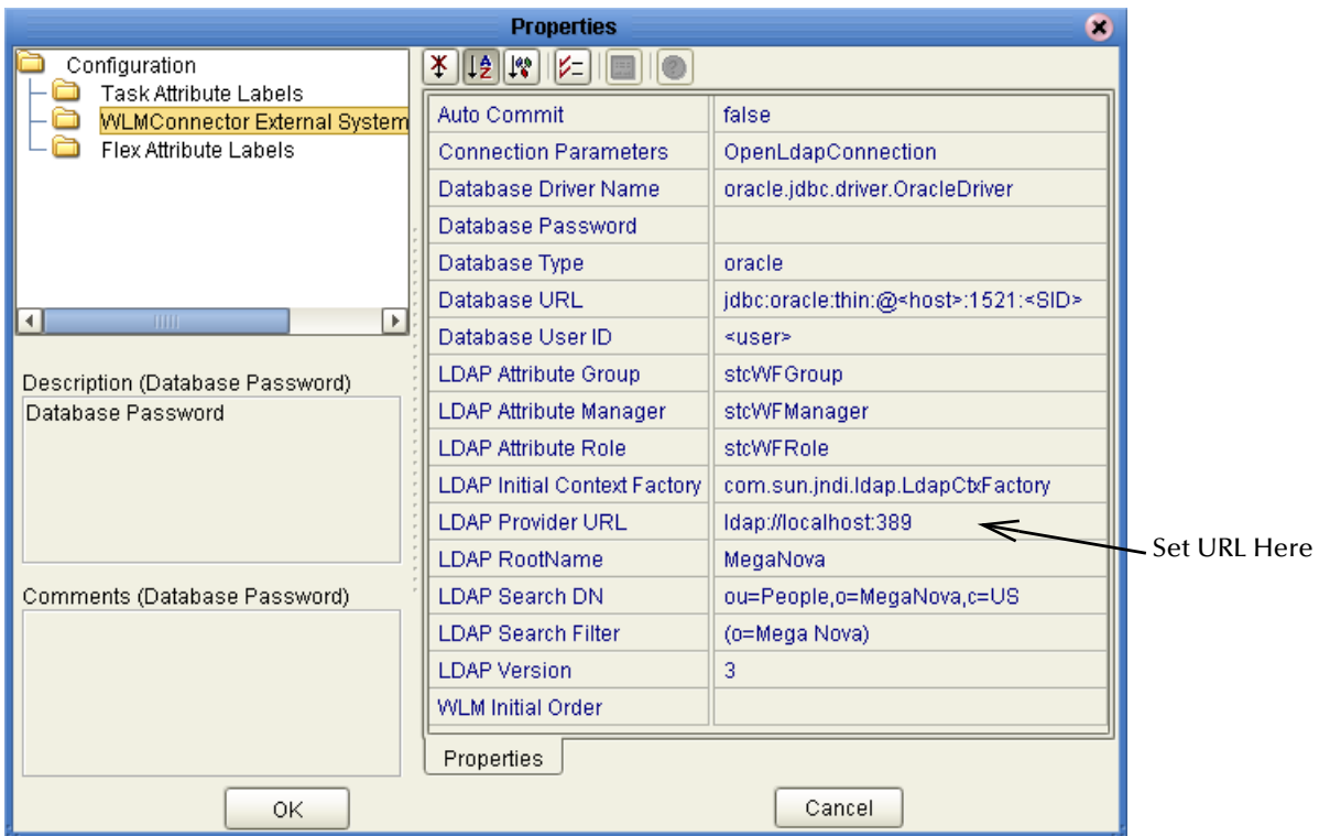
Figure 83 WLM Connector Settings
