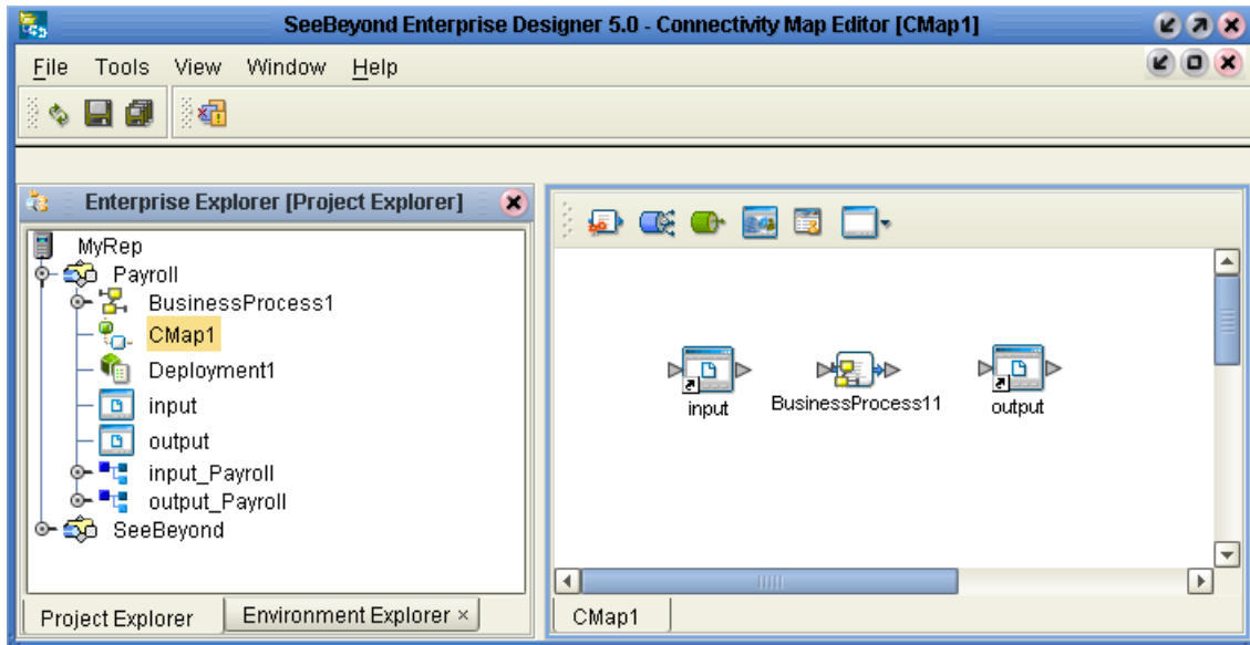
Figure 49 Connectivity Map with Business Process
