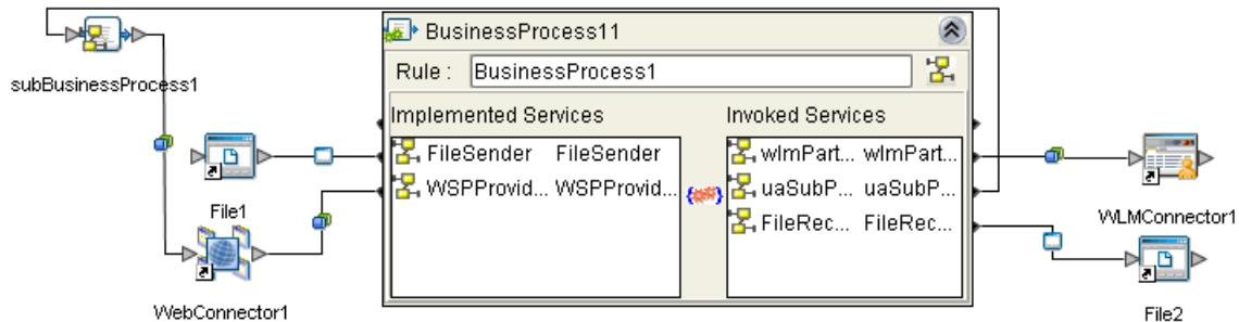
Figure 101 Completed Connectivity Map
