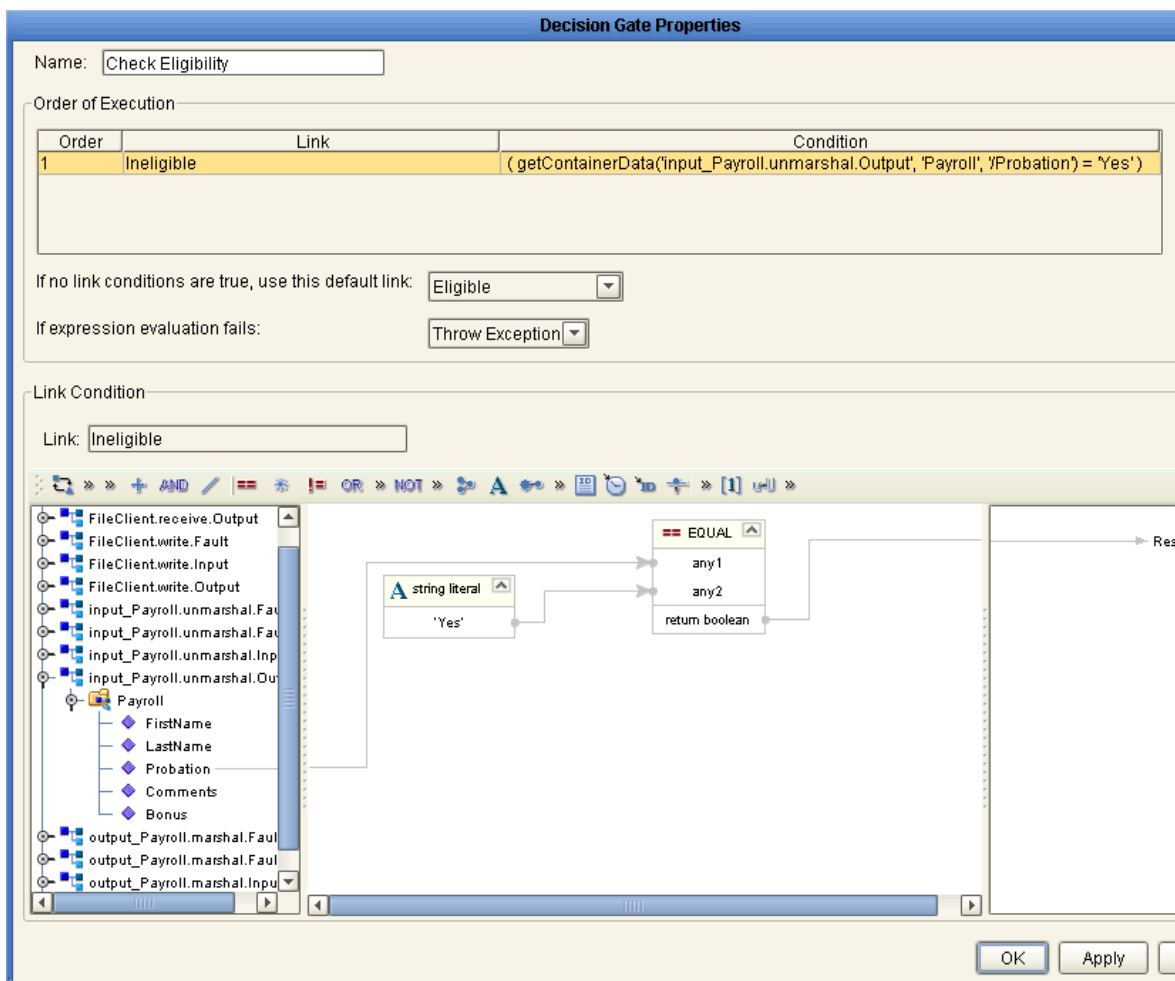
Figure 64 Completed Decision Gate Properties
