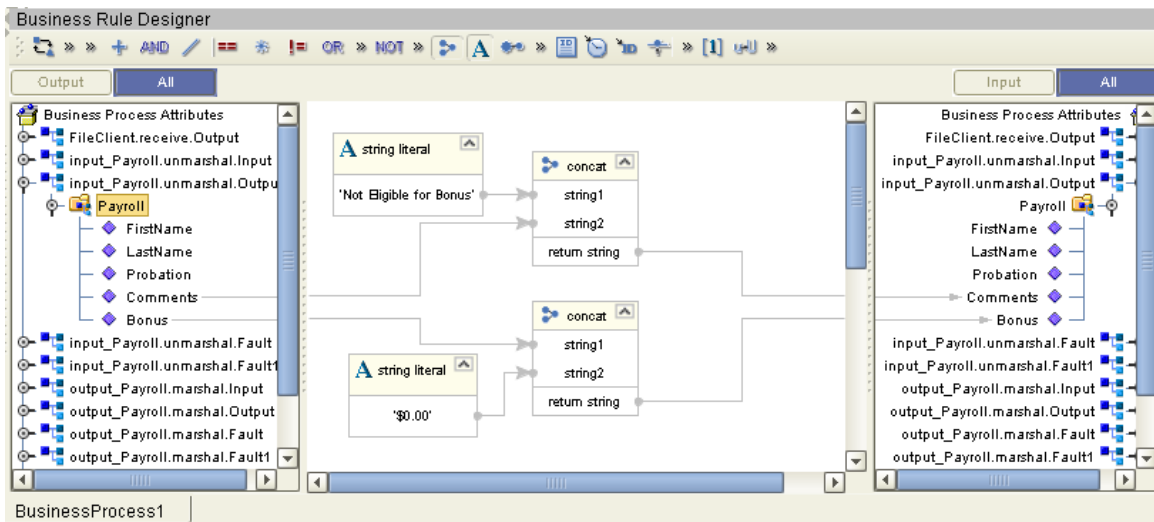
Figure 65 Update Status Activity
