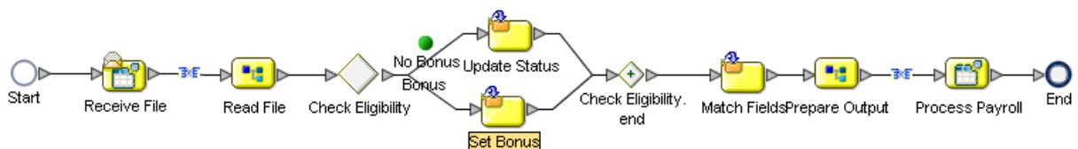
Figure 11 Sample Business Process Model
