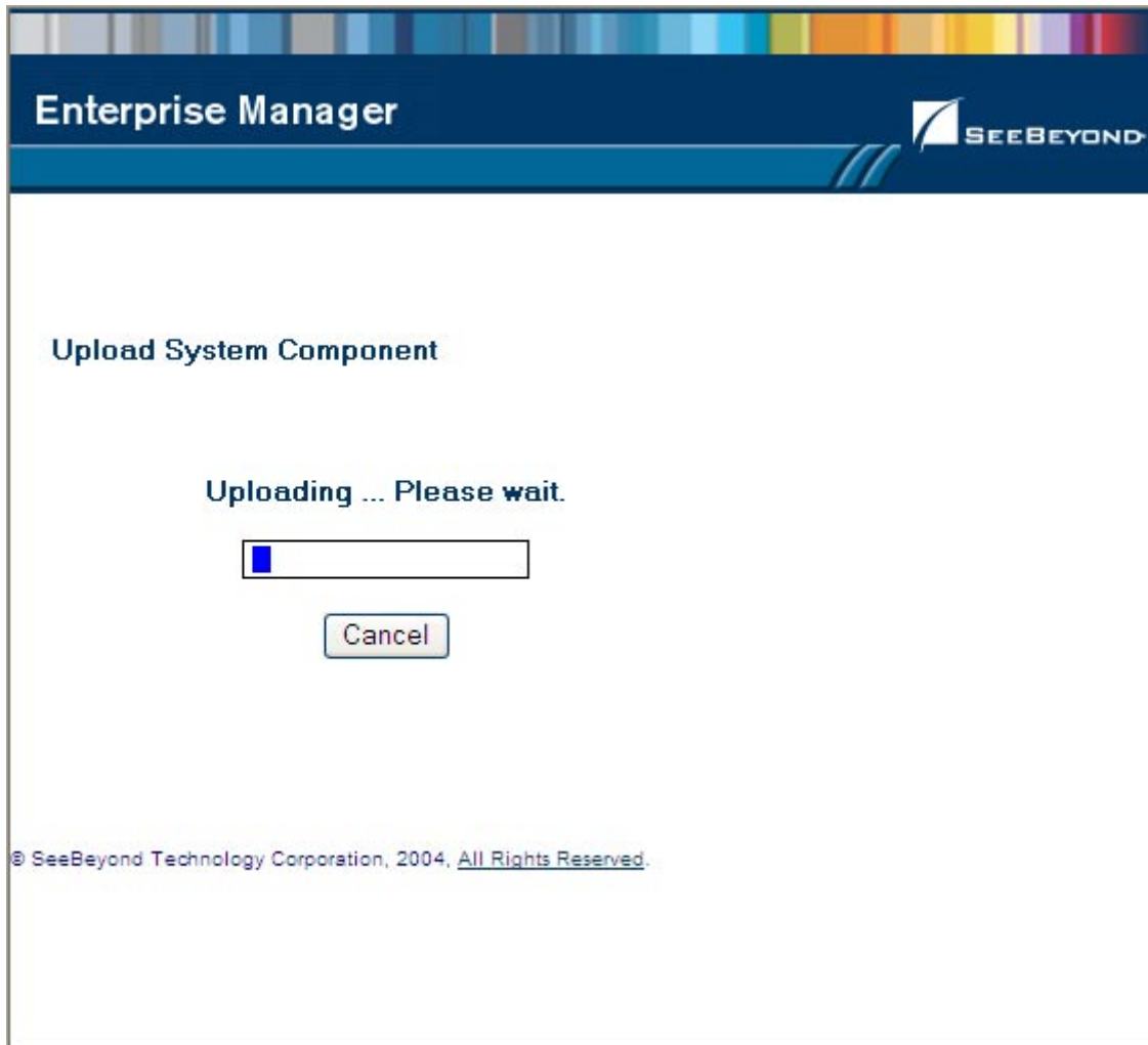
Figure 6 Upload Screen
