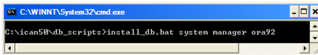
Figure 53 Install_db.bat
