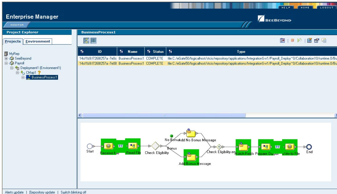
Figure 56 Monitor View
