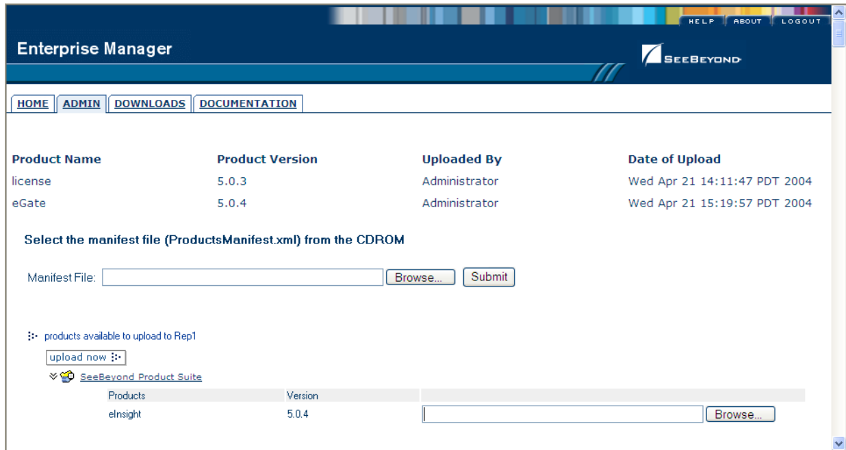
Figure 5 Upload eInsight
