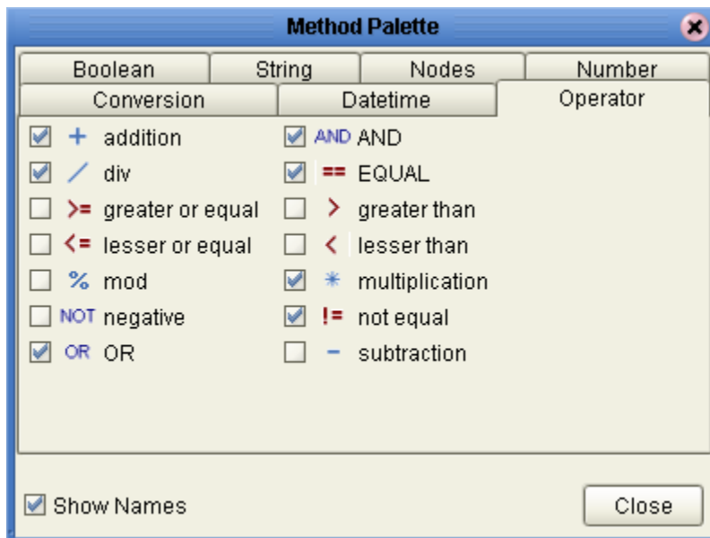
Figure 105 Method Palette: Operator Tab
