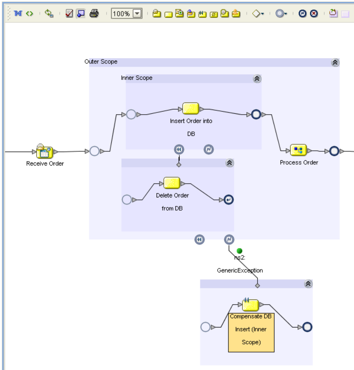
Figure 47 Example of Compensation Handling
