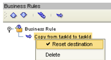
Figure 79 Reset Destination
