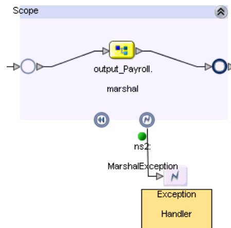
Figure 44 Configured Exception
