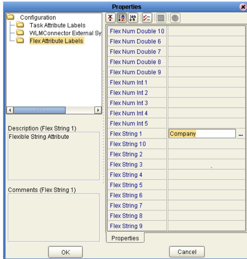
Figure 81 Flex Attributes
