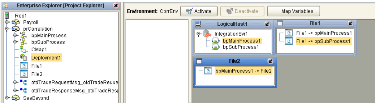
Figure 73 Deployment Profile
