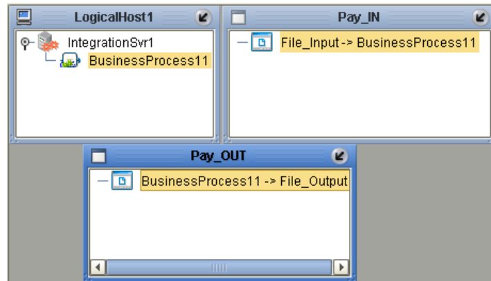
Figure 71 Deployment Profile
