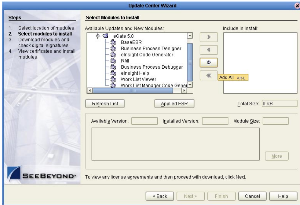
Figure 9 Select Modules
