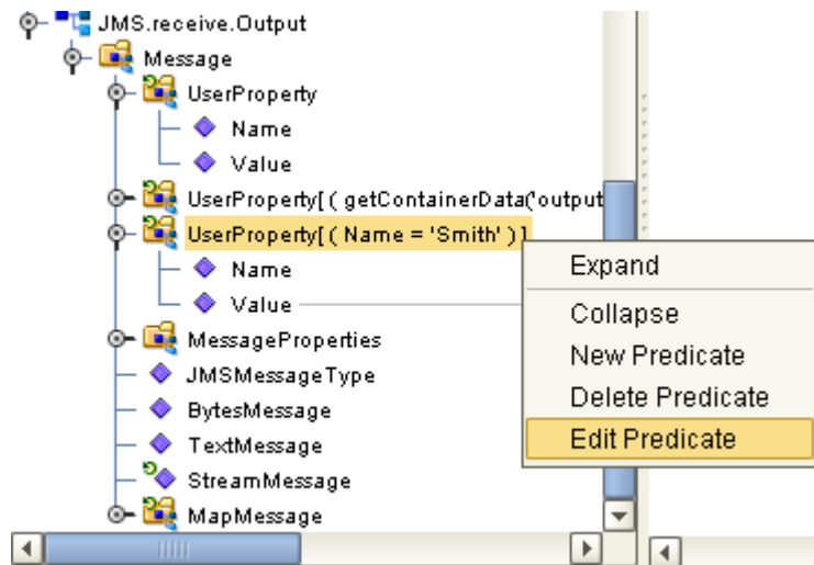
Figure 37 Edit Predicate
