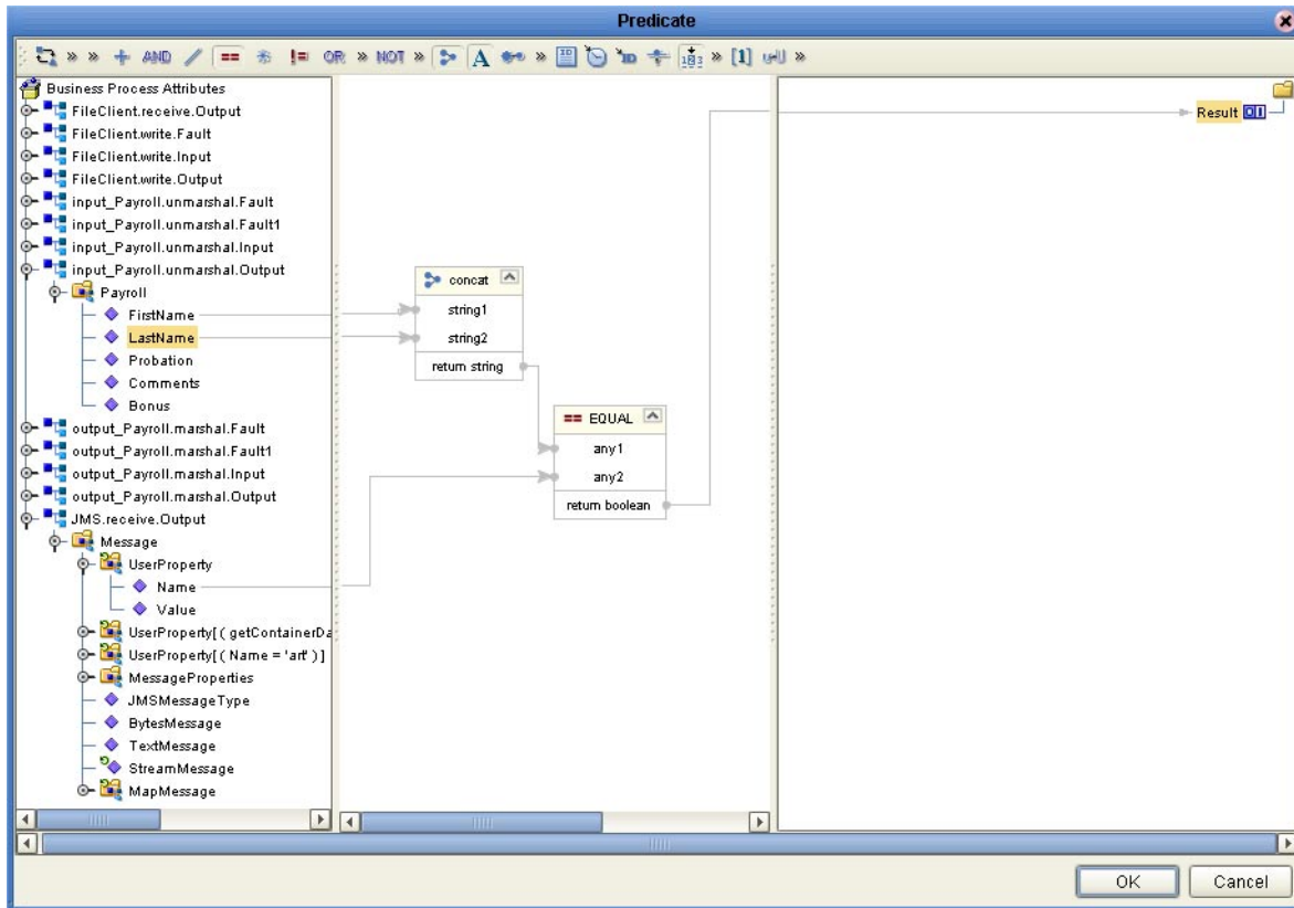
Figure 38 Predicate Editor
