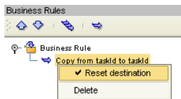
Figure 20 Delete Rule
