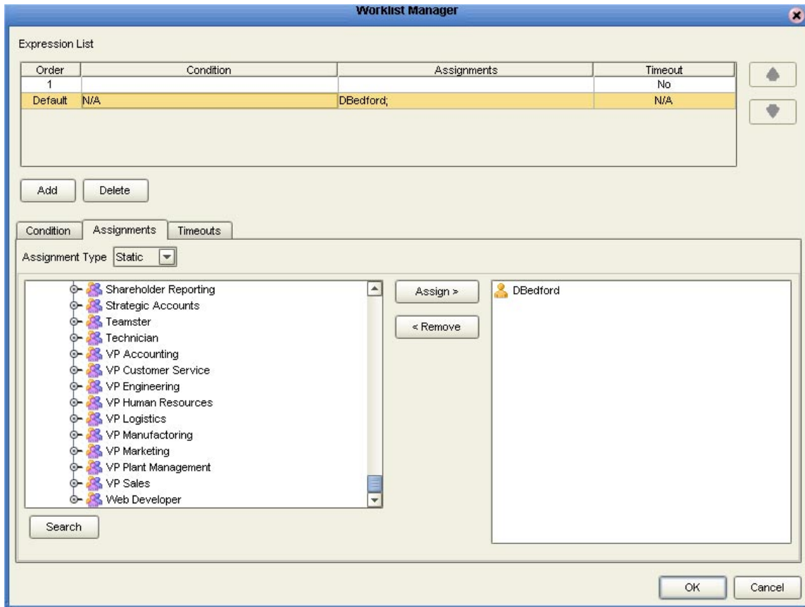
Figure 100 Assign Users
