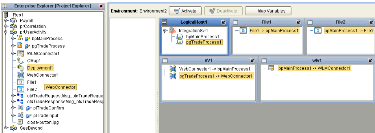
Figure 103 User Activity Deployment Profile
