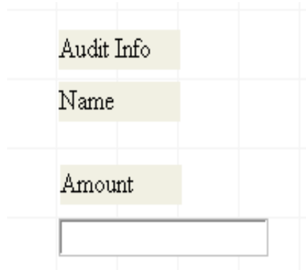
Figure 91 auditPage Layout
