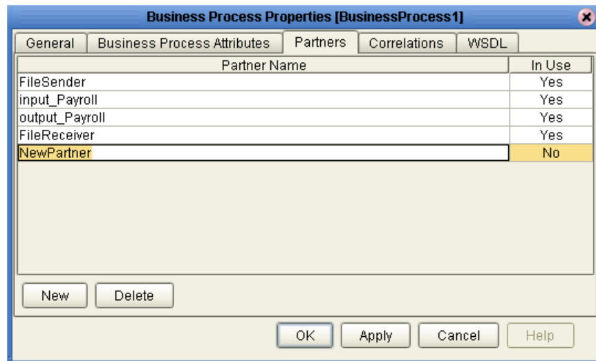
Figure 25 New Partner
