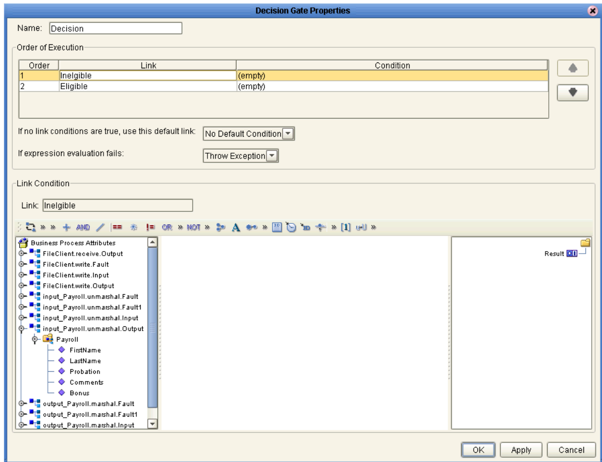
Figure 63 Decision Properties
