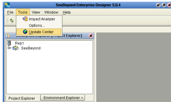
Figure 8 Update Center
