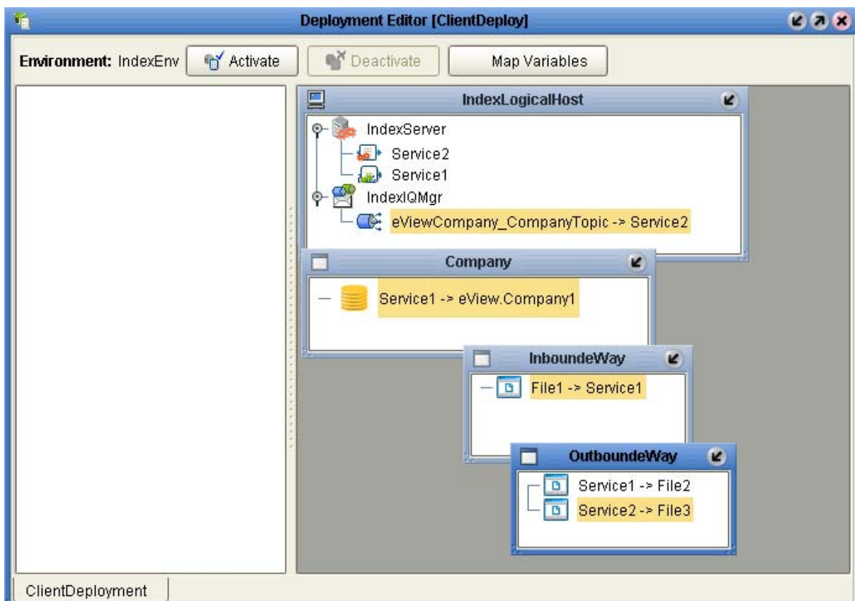
Figure 71 Mapped Client Components in the Deployment Editor
