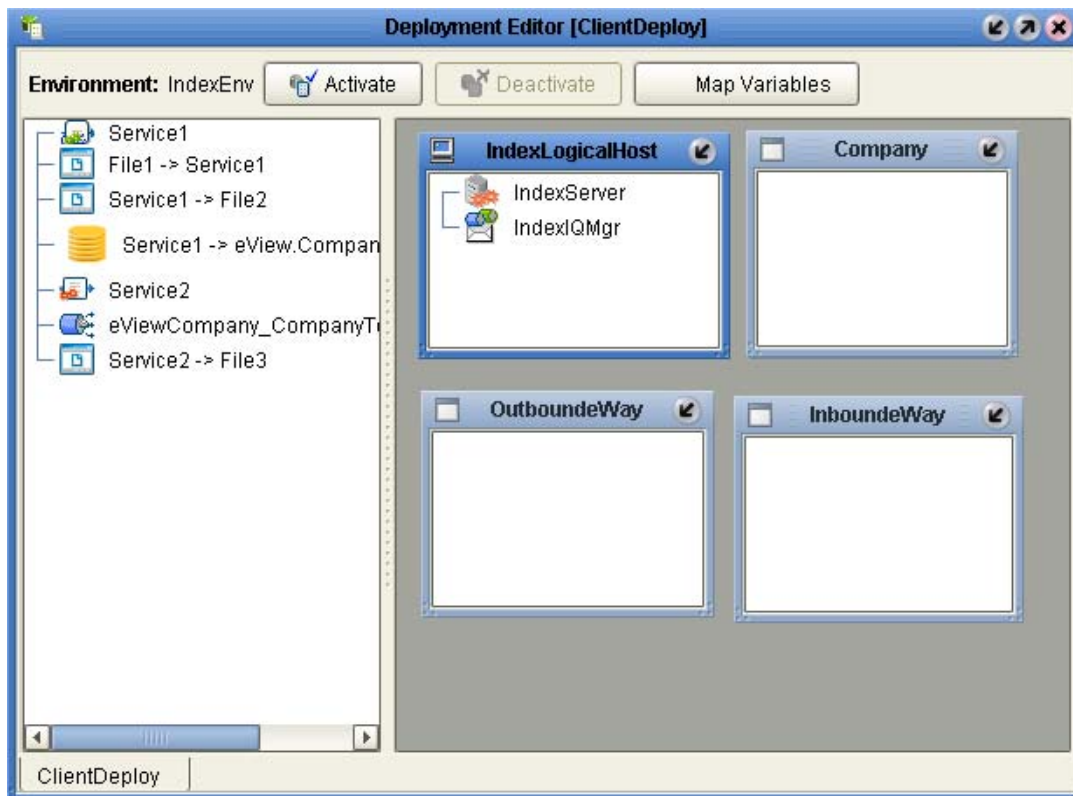
Figure 70 Deployment Editor Window - Client Project
