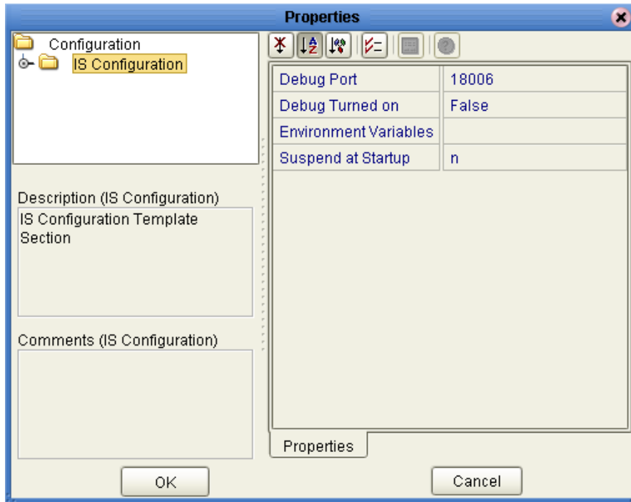
Figure 62 Integration Server Configuration Properties
