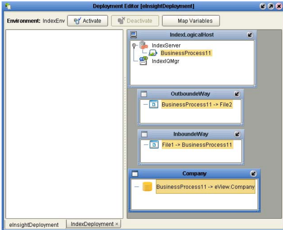
Figure 74 Mapped Client Components in the Deployment Editor
