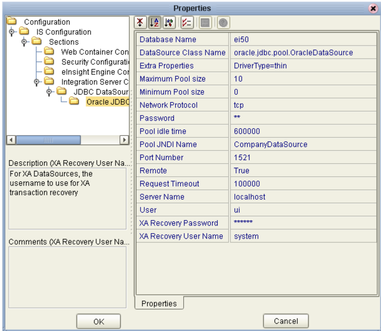
Figure 61 Integration Server Properties
