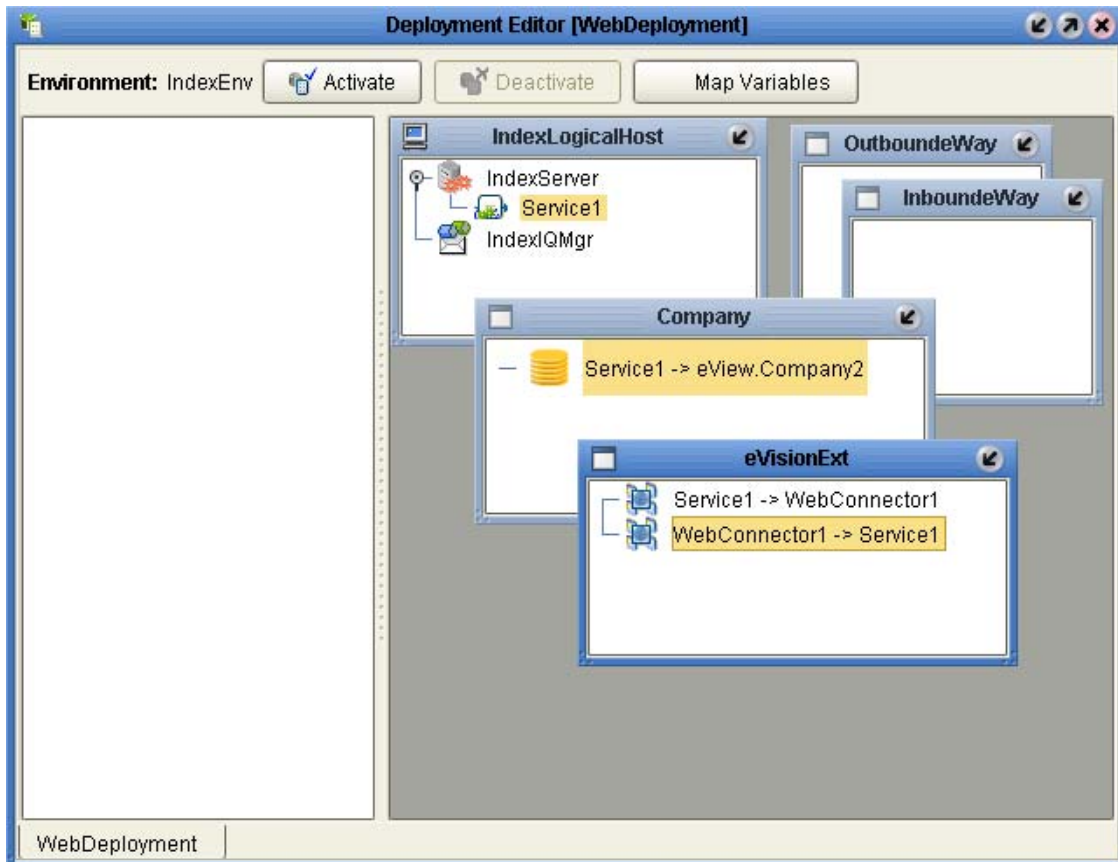
Figure 77 Mapped Client Components in the Deployment Editor
