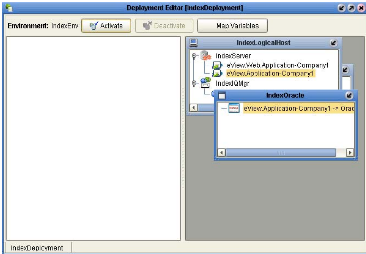
Figure 68 Mapped eView Components in the Deployment Editor
