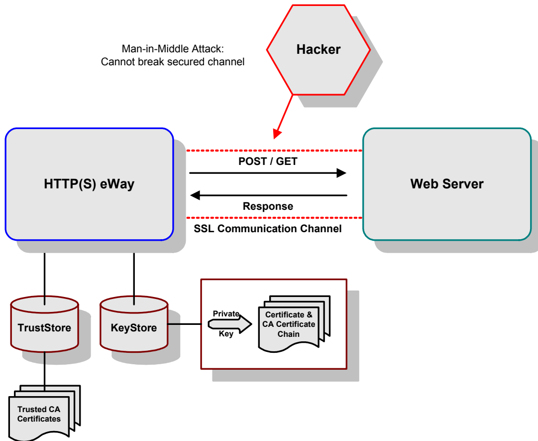
Figure 38 General SSL Operation: HTTP(S) eWay
