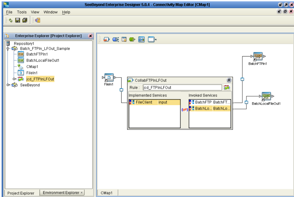
Figure 64 Connectivity Map - Binding the Project components
