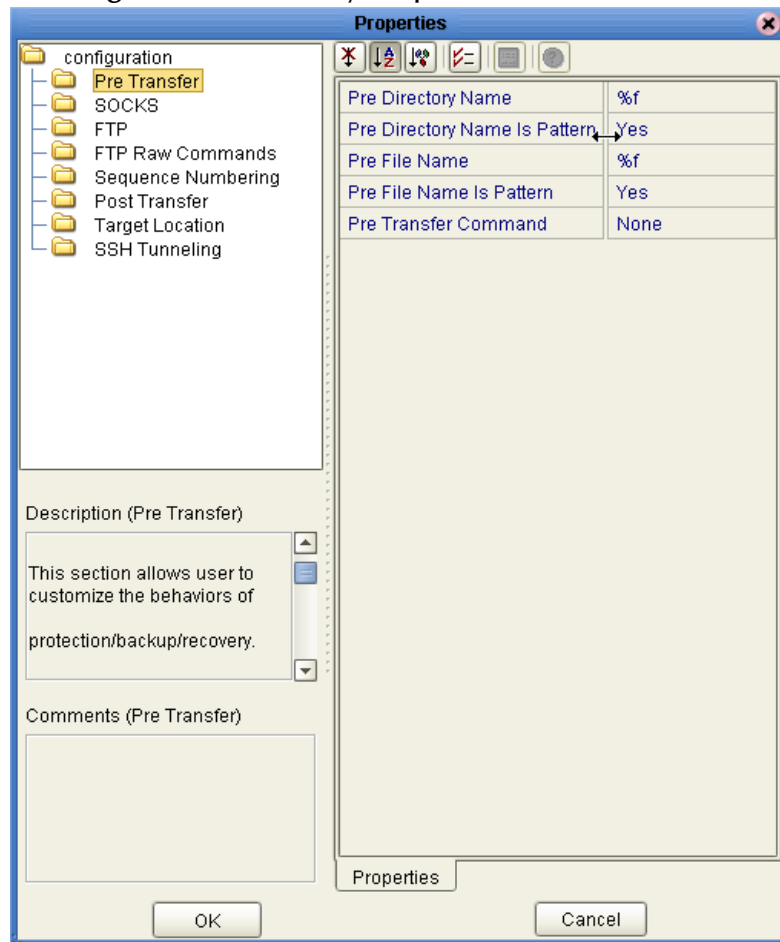
Figure 3 Batch eWay Properties Editor
