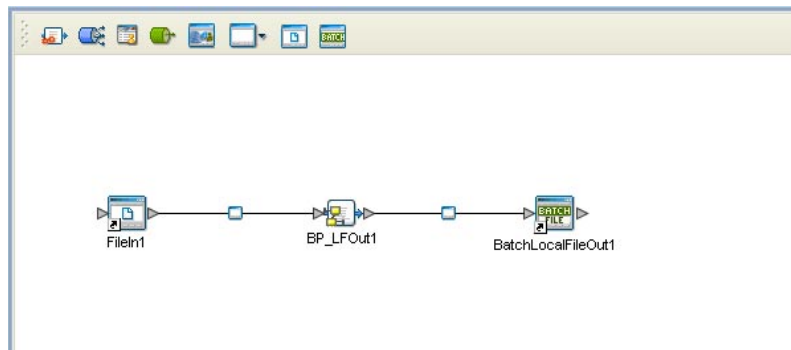
Figure 52 Connectivity Map - Connecting the Project's Components
