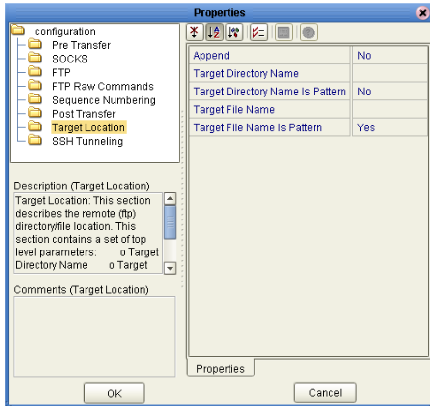
Figure 10 BatchFTP Properties - Target Location section
