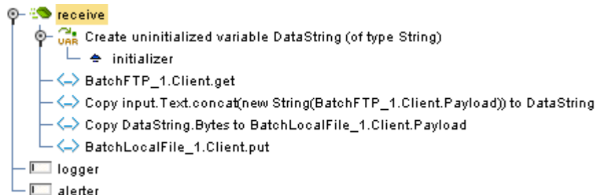
Figure 58 jcd_Passthru Business Rules
