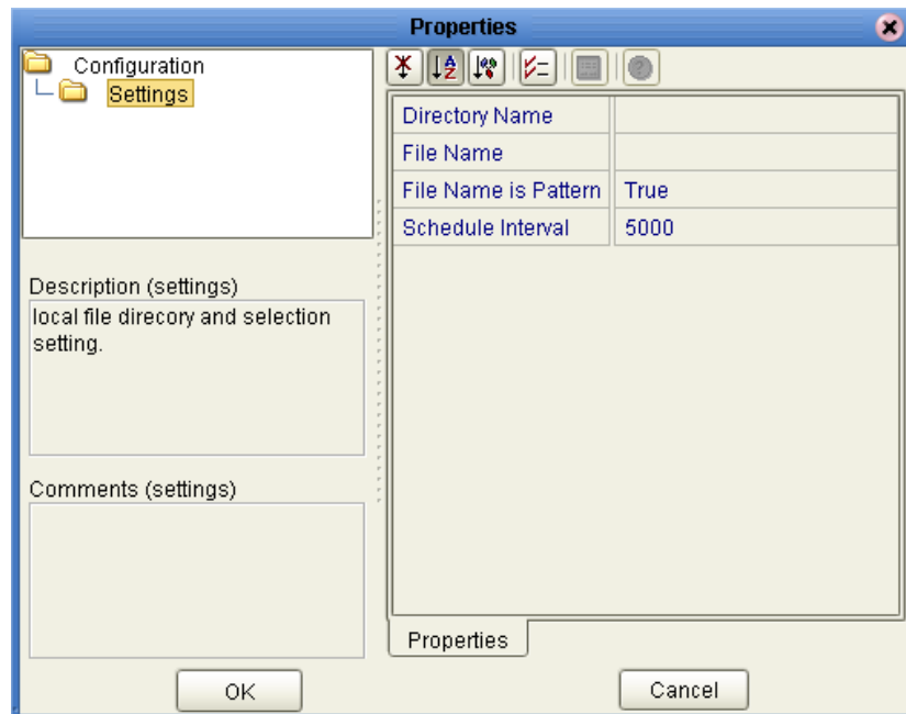
Figure 22 BatchInbound Properties - Settings section
