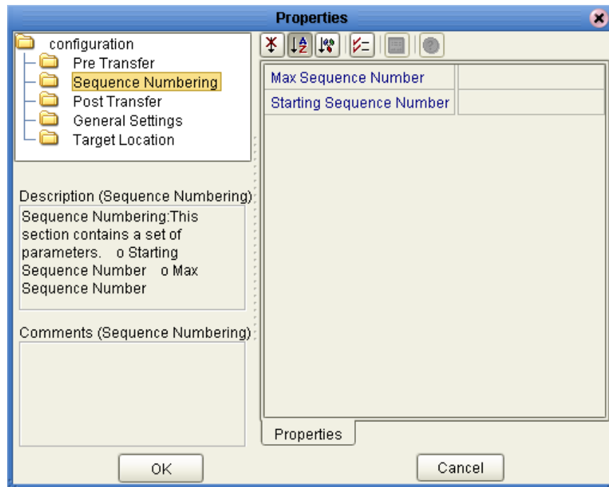
Figure 16 BatchLocalFile Properties - Sequence Numbering section
