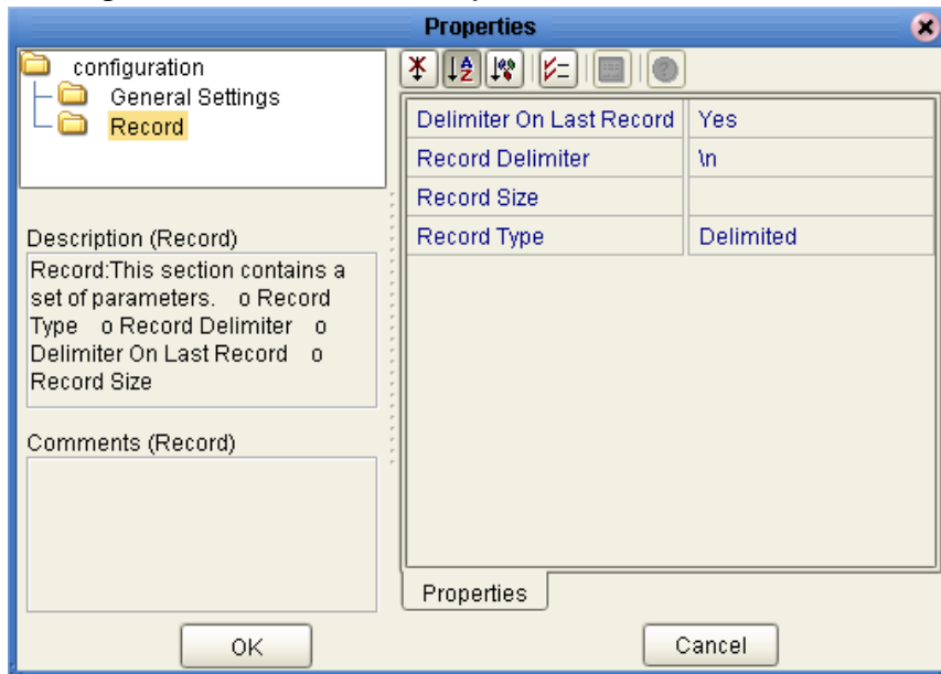
Figure 21 BatchRecord Properties - Record section
