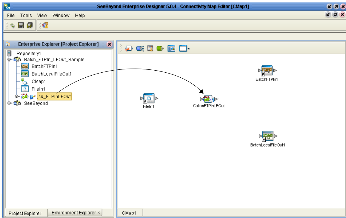
Figure 63 Connectivity Map - Binding the Project components
