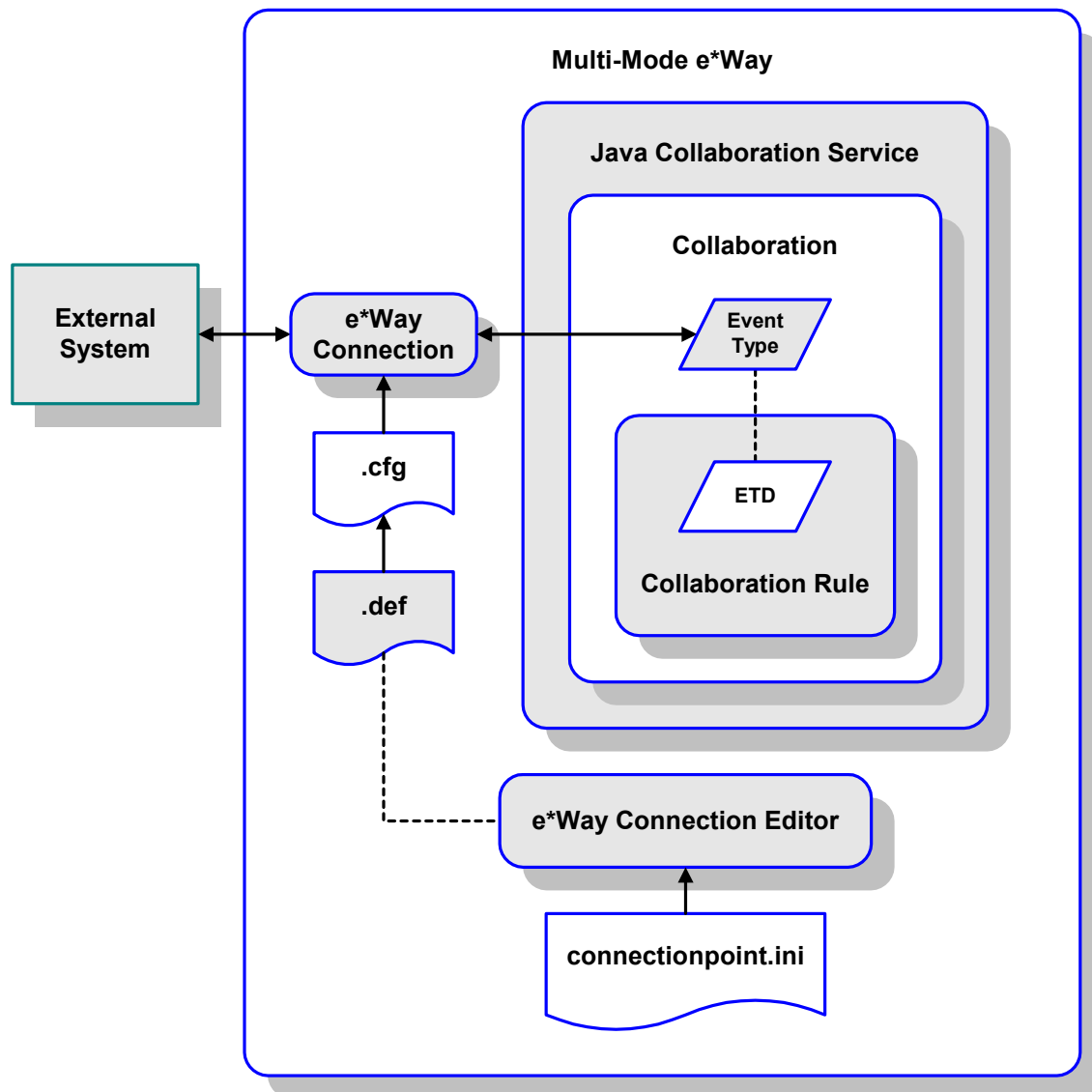
Figure 110 e*Way Connection Establishment
