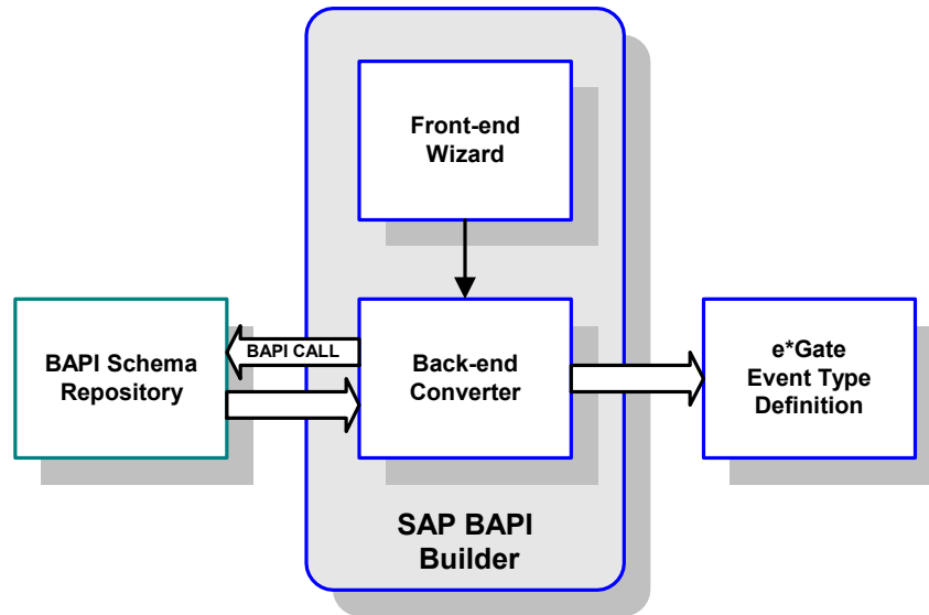
Figure 107 SAP BAPI Wizard
