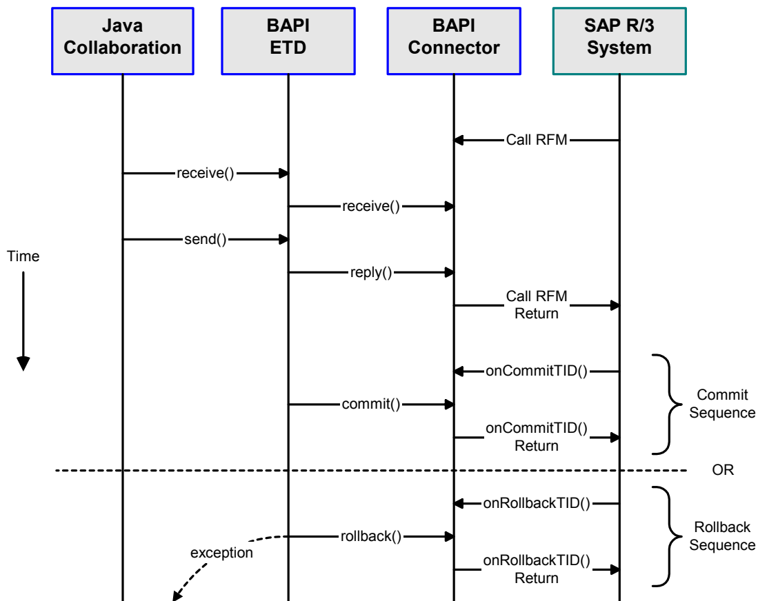
Figure 100 Transactional RFC Server Sequence
