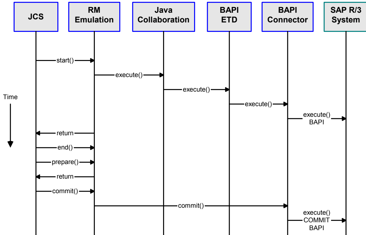
Figure 94 XA-Compliant Client Sequence
