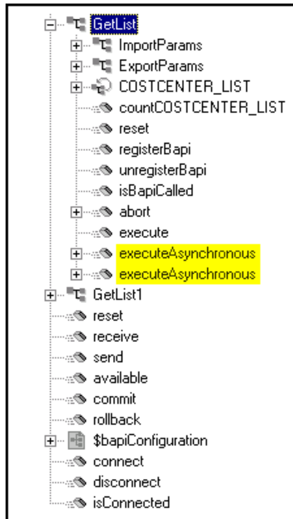
Figure 39 tRFC Connections (Client)
