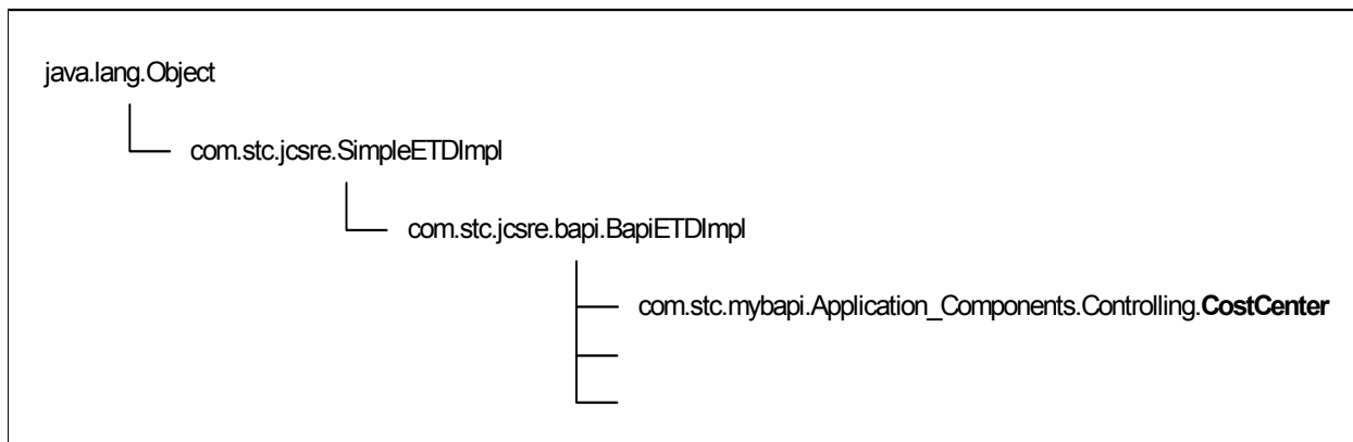
Figure 113 CostCenter Class Hierarchy
