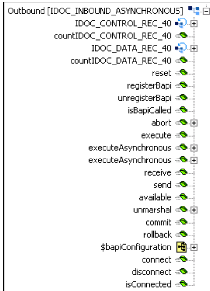
Figure 68 IDoc Client Sample ETD - IDOC_INBOUND_ASYNCHRONOUS
