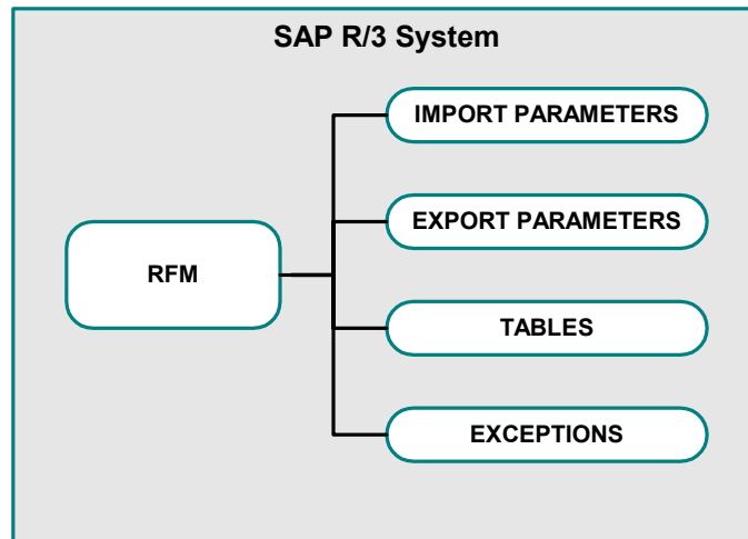
Figure 90 Remote Function Module
