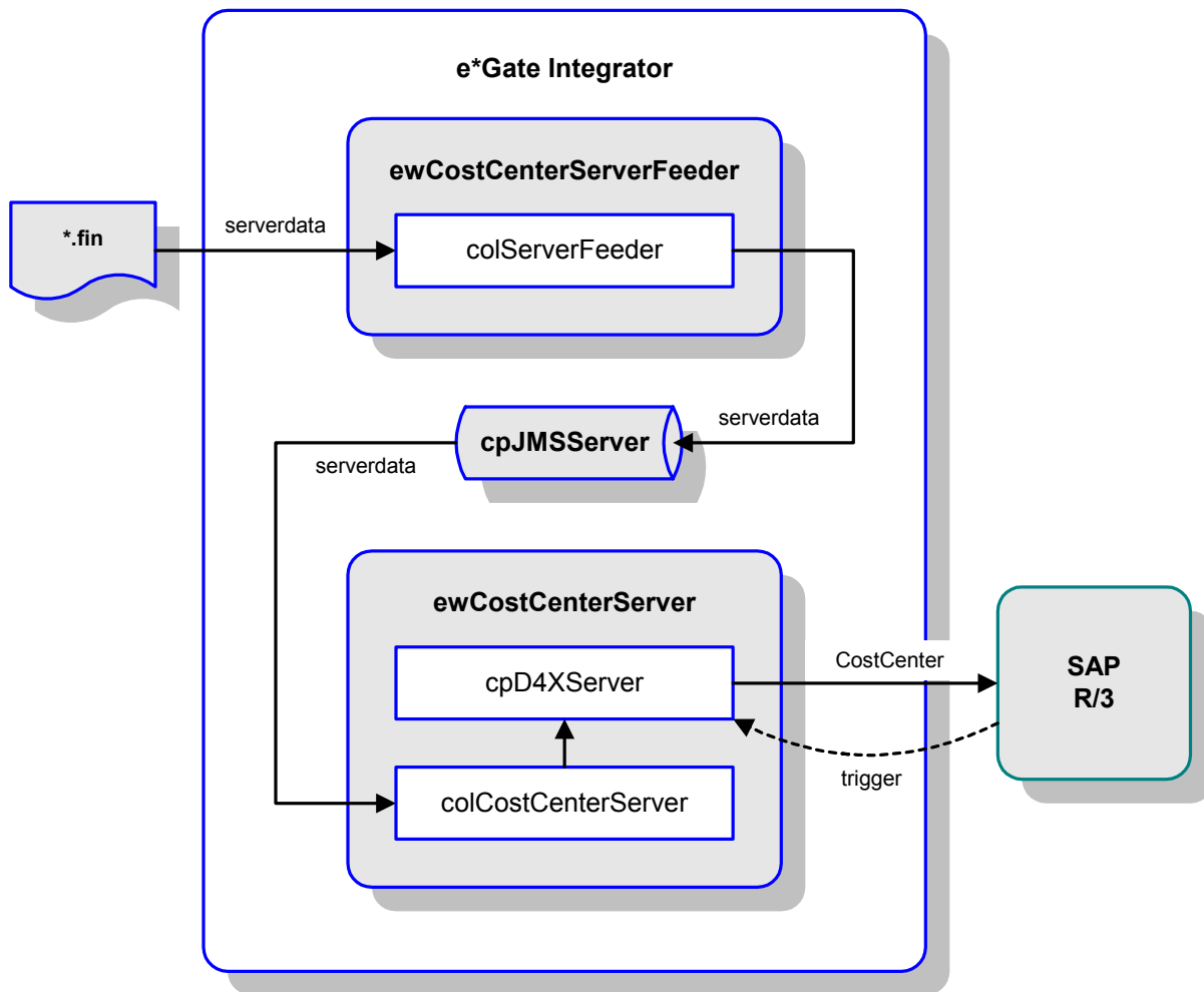
Figure 61 BAPI Sample - Server Mode
