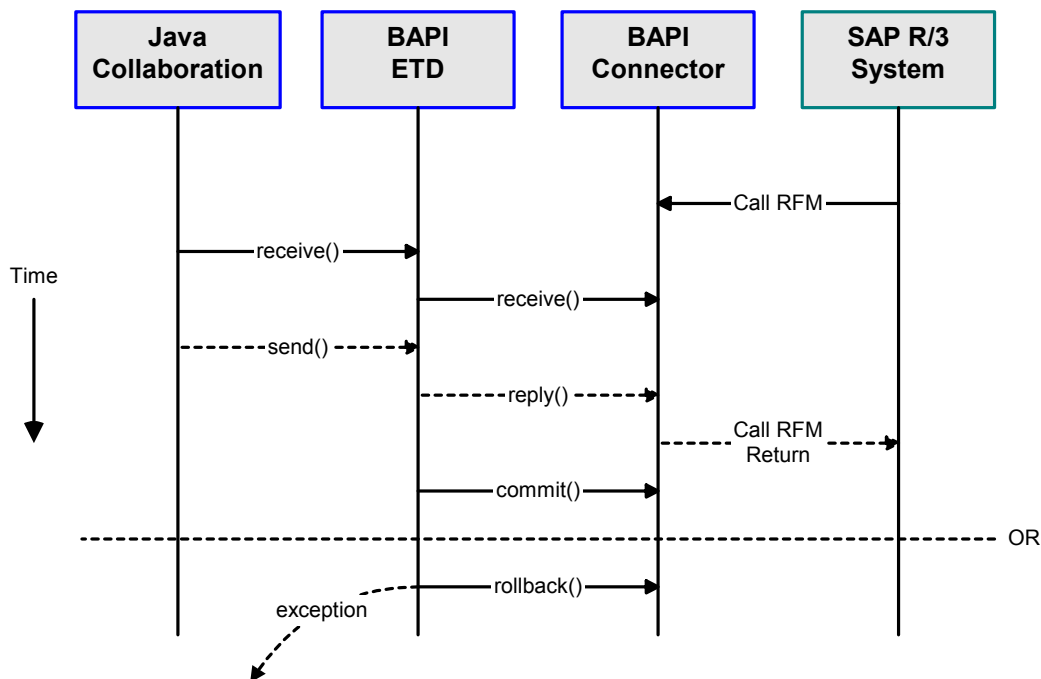
Figure 99 Internal RFC Server Sequence
