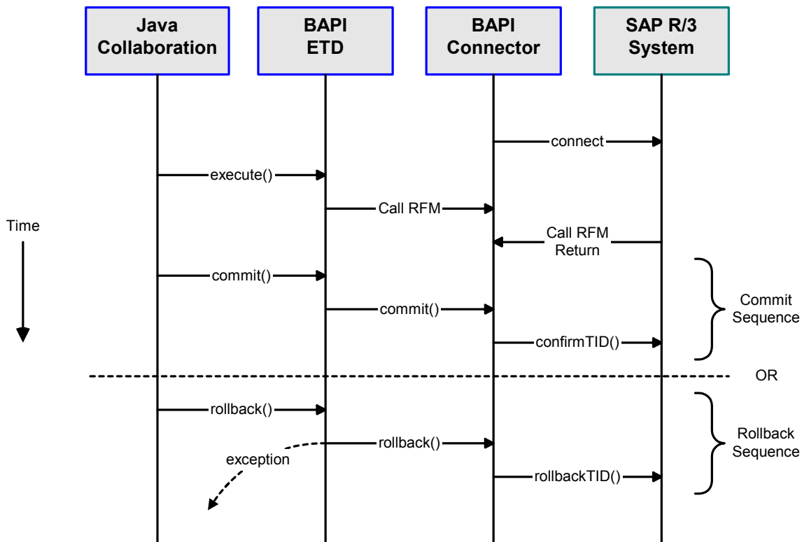
Figure 96 Transactional RFC Client Sequence
