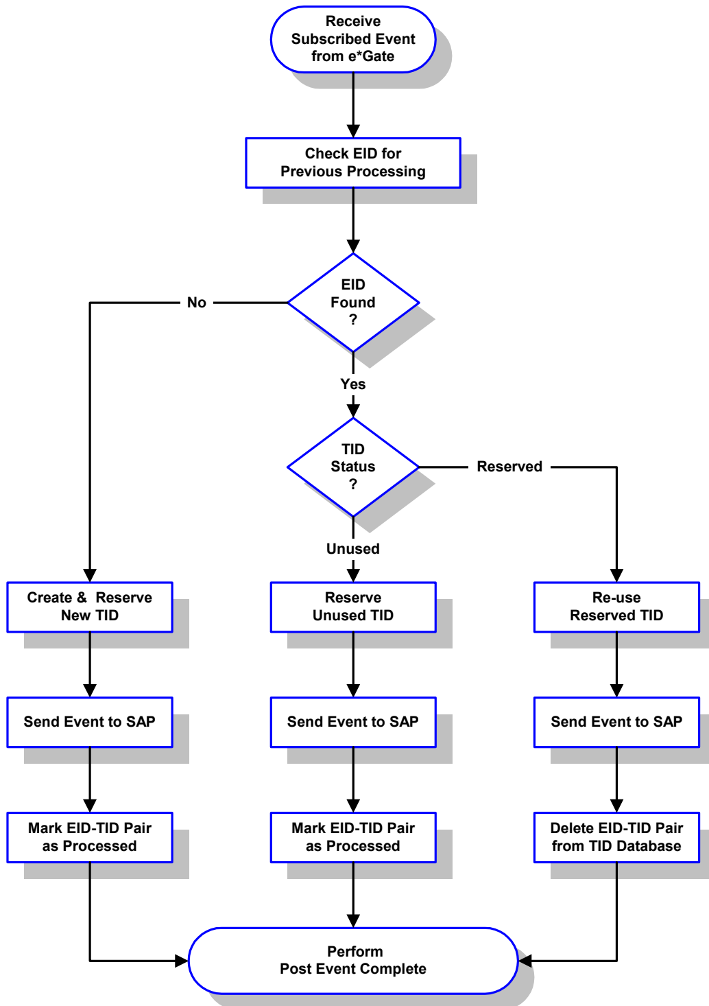
Figure 95 tRFC Client Mode Process Flow
