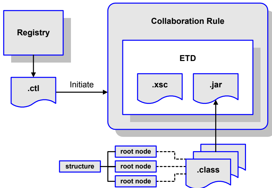
Figure 108 Event Type Definitions
