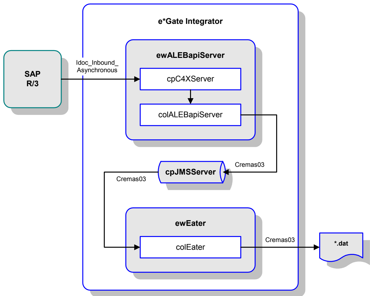
Figure 71 IDoc Sample - Server Mode
