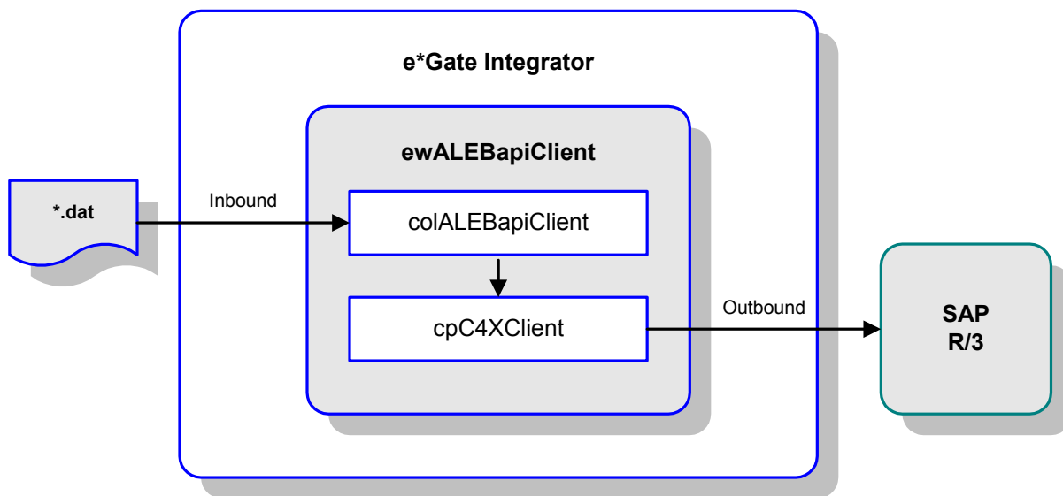
Figure 66 IDoc Sample - Client Mode
