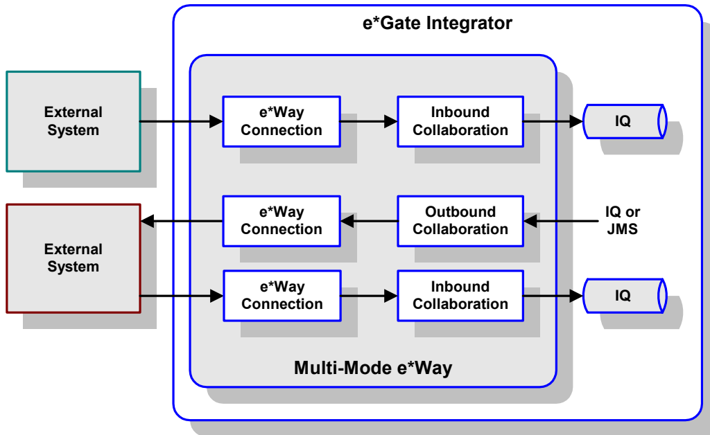
Figure 102 e*Way within e*Gate Integrator
