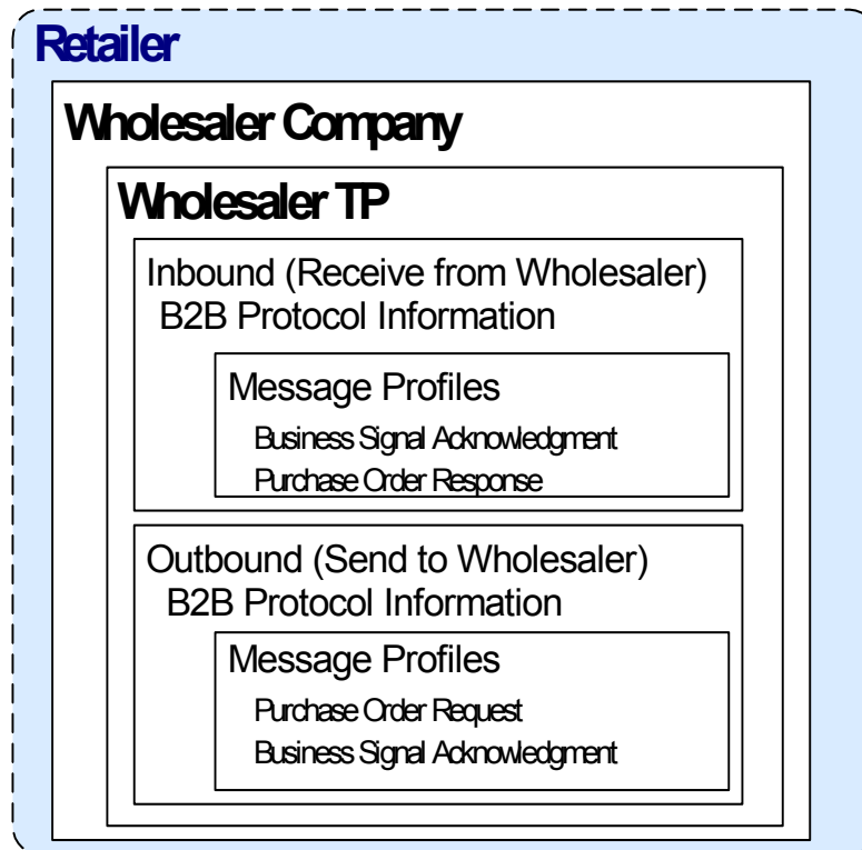
Figure 69 Wholesaler Trading Partner Configuration on the Retailer Company
