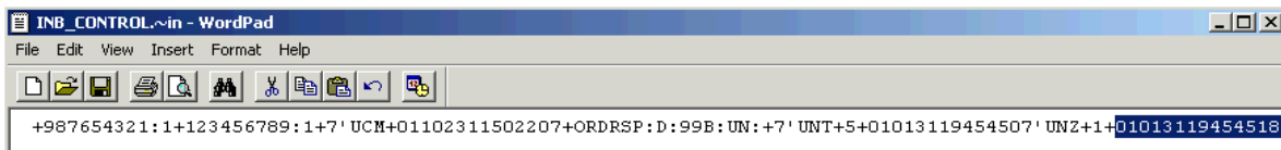
Figure 65 Control Message: Incrementing the UNZ Control Number
