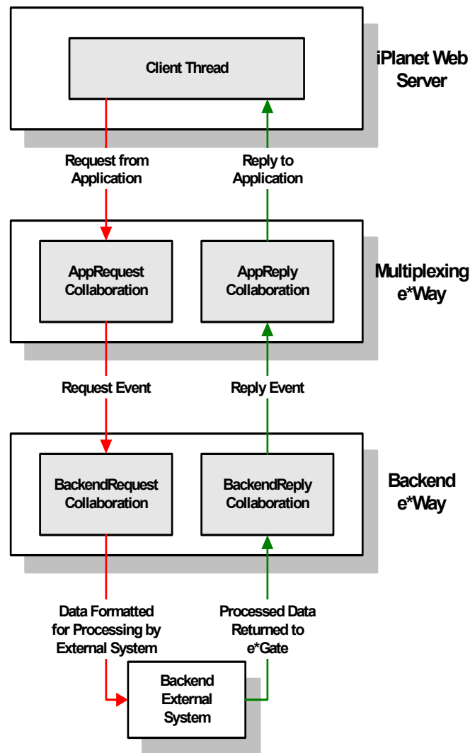
Figure 1 Overview of the iPlanet e*Way implementation
