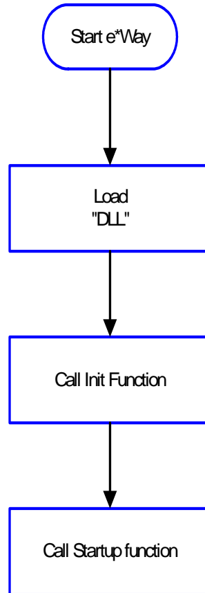
Figure 11 Initialization Functions
