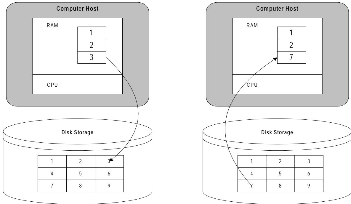
Figure 20 Memory Swapping
