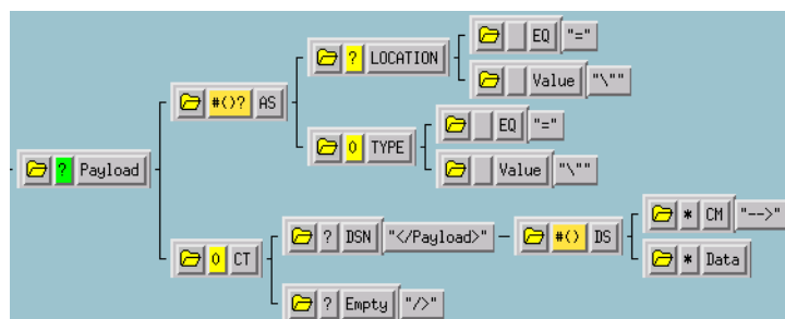
Figure 117 XML Attribute Type
