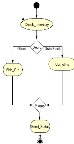
Figure 69 ProcessOrder BP with Dynamic Sub-Process
