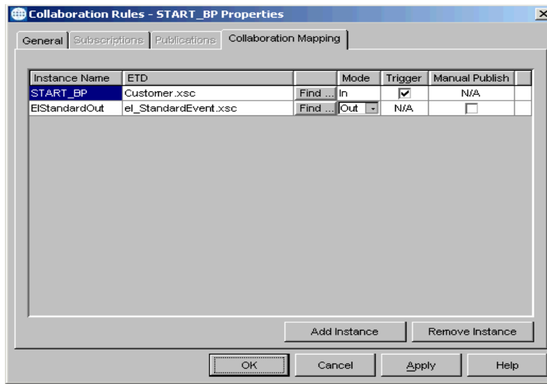
Figure 77 Start_BP Properties, Collaboration Mapping Tab
