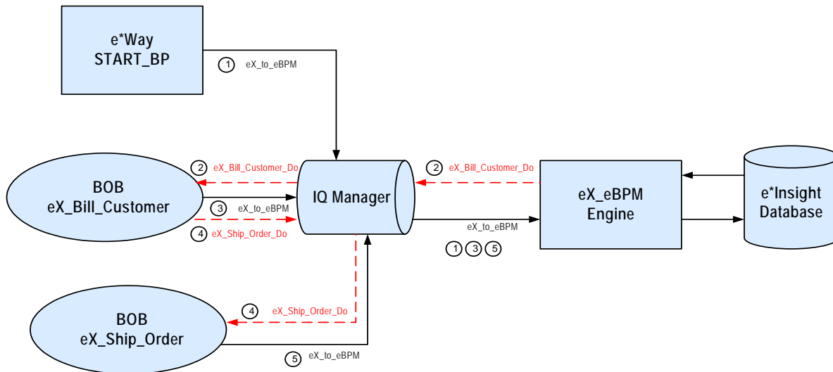
Figure 71 e*Insight Data Flow Diagram
