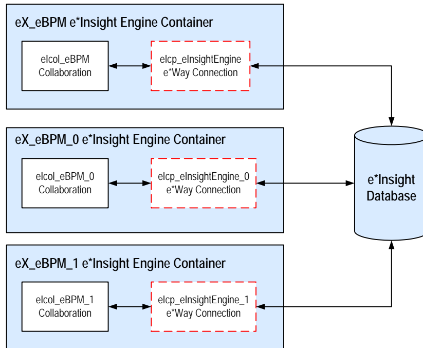
Figure 96 Multiple Engine Containers with a Single Engine
