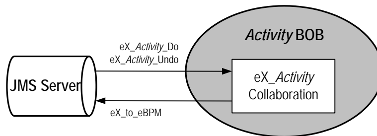
Figure 10 Activity BOB Detail
