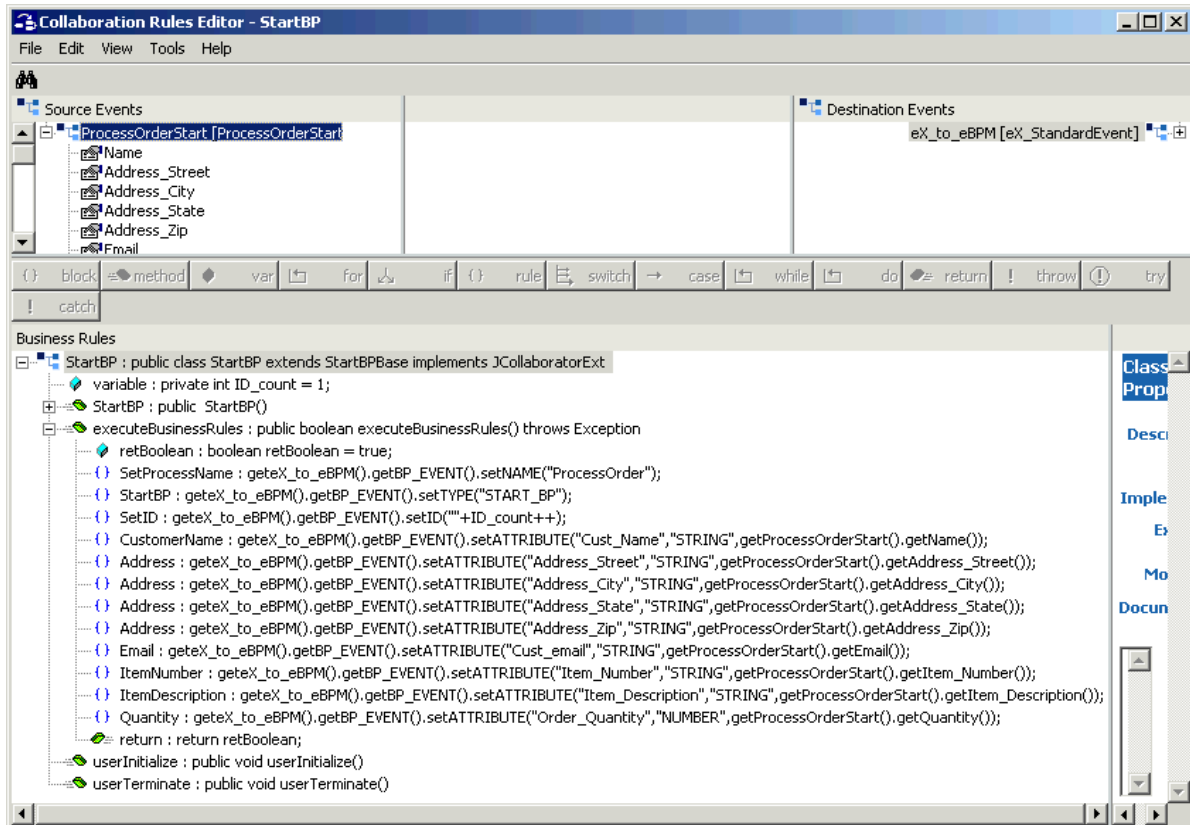
Figure 150 START_BP CRS (Java)
