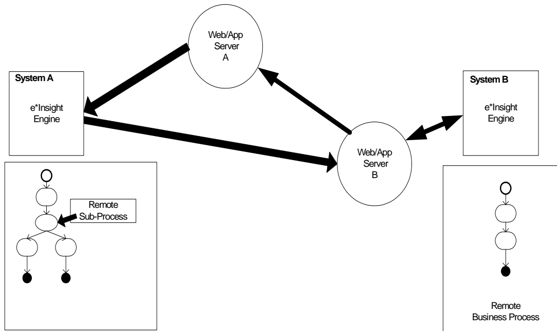
Figure 90 Remote Sub-Process Overview
