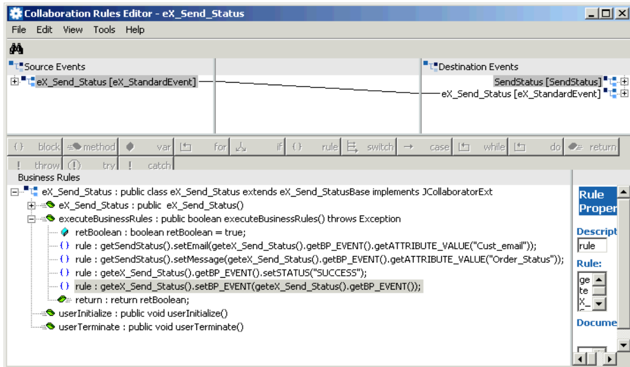
Figure 156 eX_Send_Status.xsc CRS (Java)
