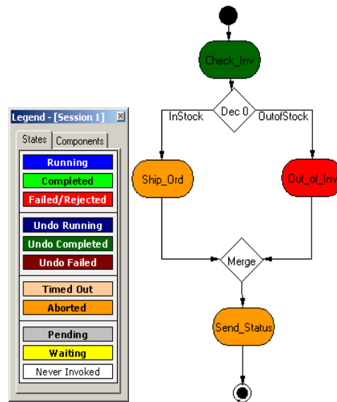
Figure 161 Manual Undo Completed BPI Diagram
