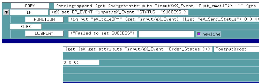
Figure 153 eX_Send_Status.tsc CRS (Monk)
