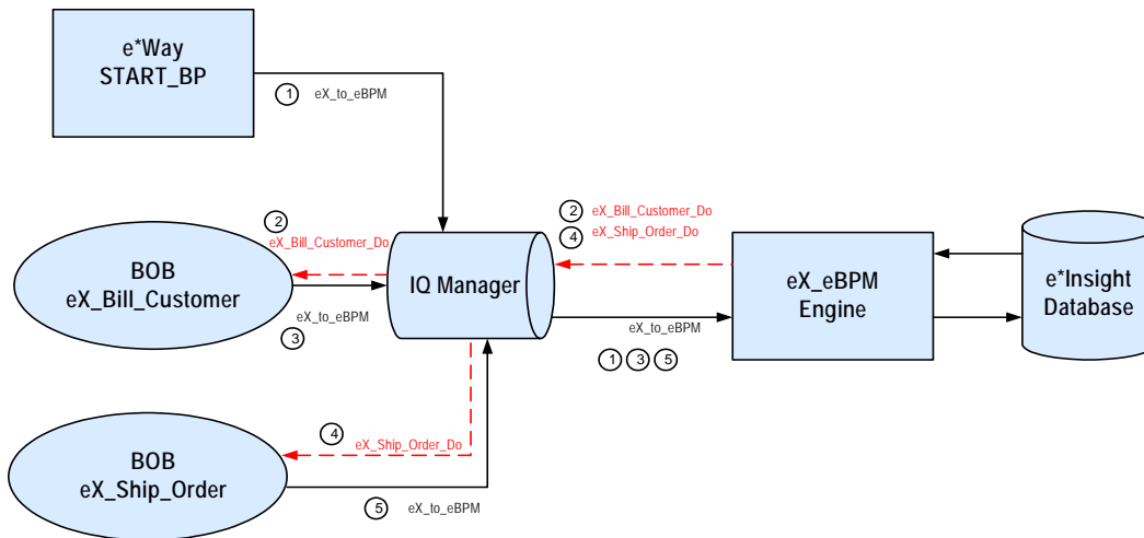
Figure 70 e*Insight Data Flow Diagram
