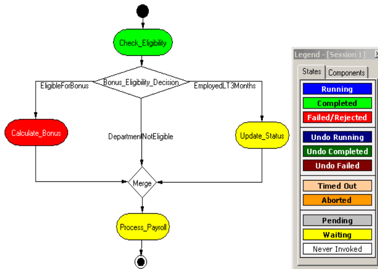
Figure 47 Attribute Repair—Failed BPI Diagram
