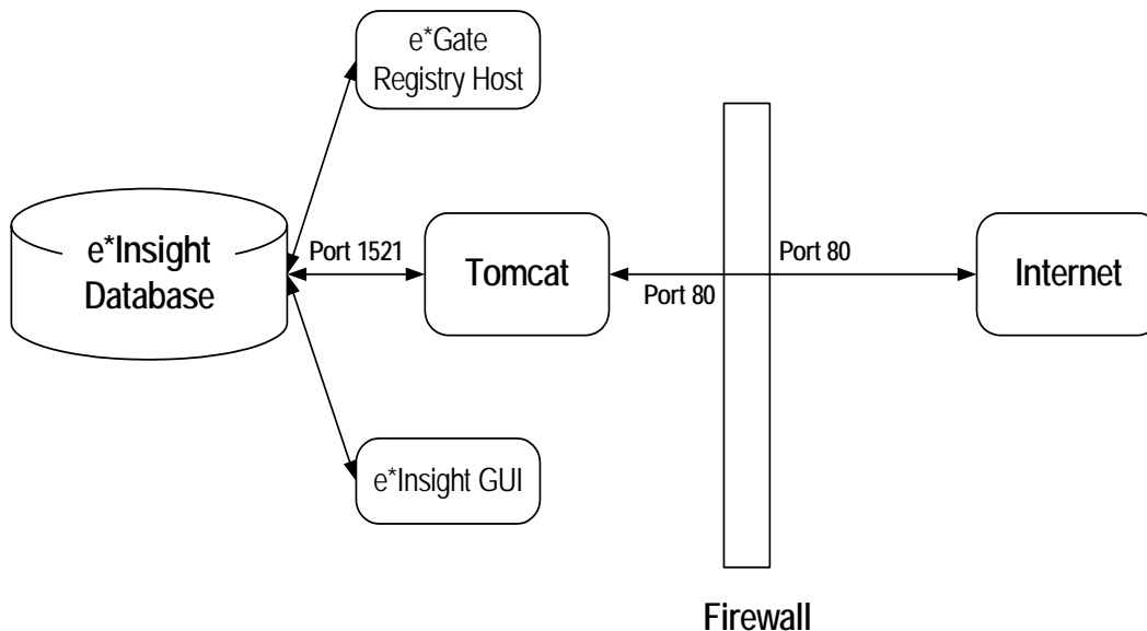
Figure 91 e*Insight and Tomcat Deployment
