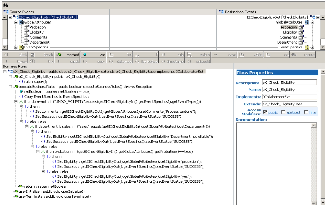
Figure 25 eX_Check_Eligibility.xpr CRS (Java)
