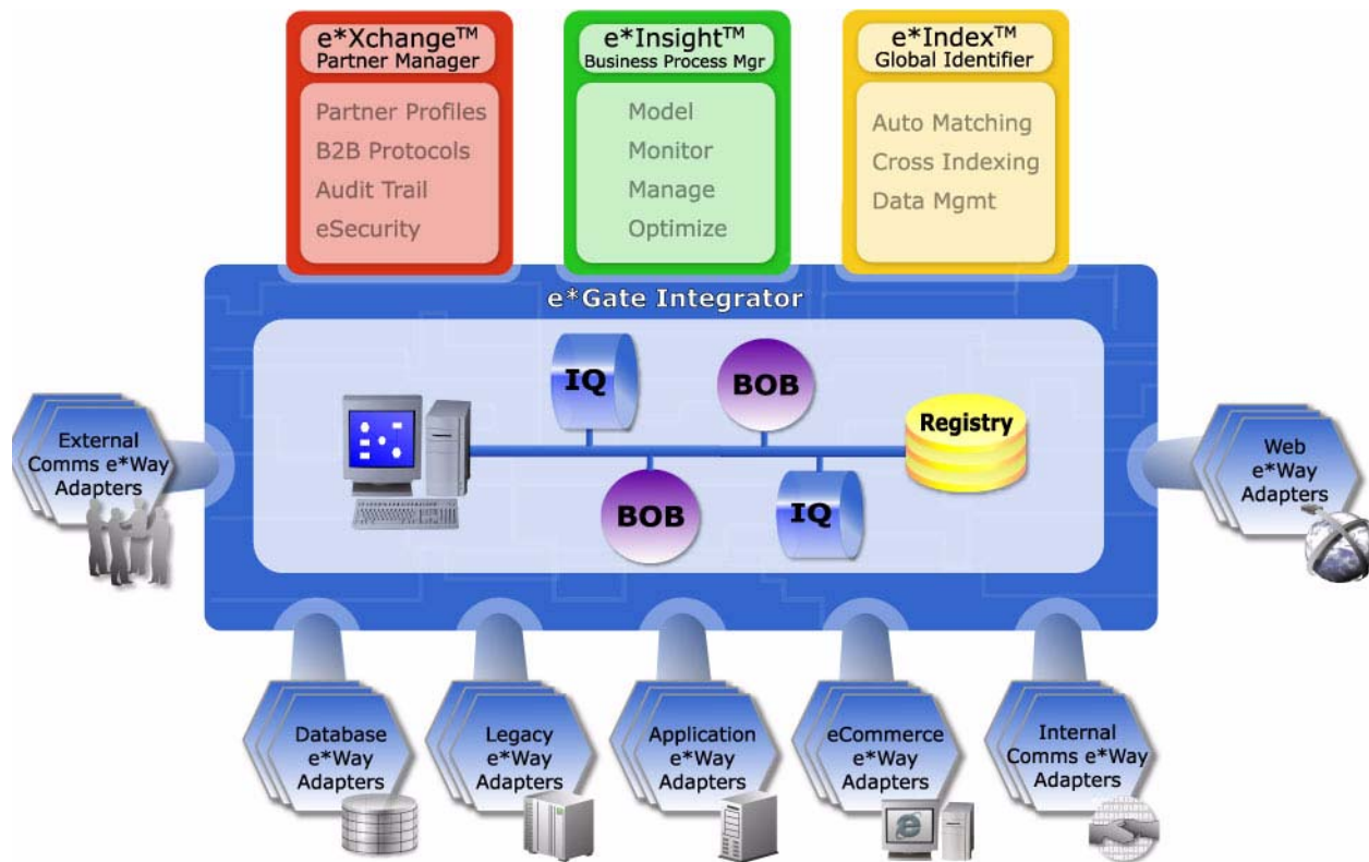
Figure 1 Oracle eBusiness Integration Suite
