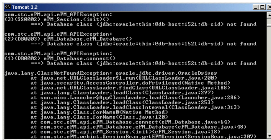
Figure 150 Classes12.zip missing from classpath: Tomcat Error
