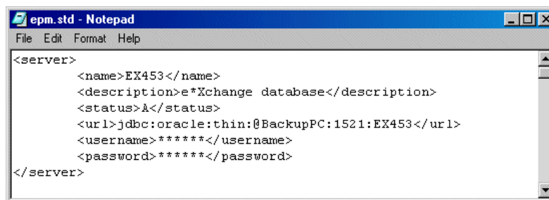
Figure 32 Sample epm.std File
