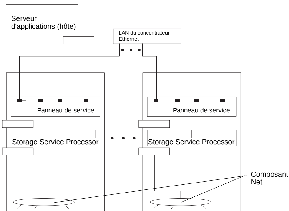
FIGURE 4-1 Unités multiples sans l'option Sun StorEdge Remote Response
