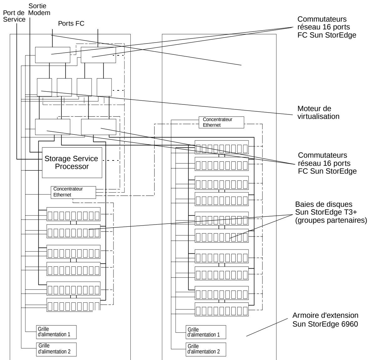
FIGURE 1-4 Système Sun StorEdge 6960
