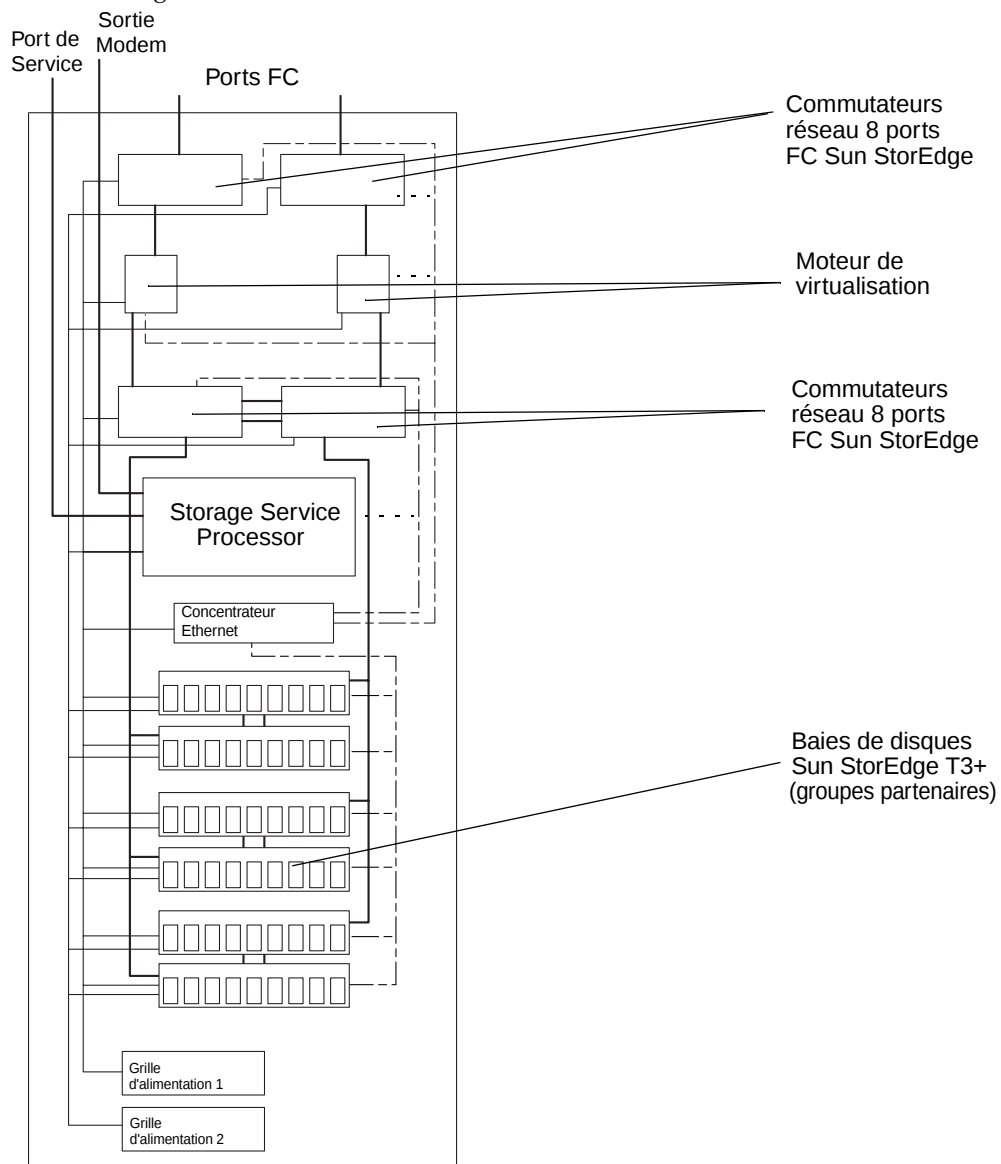
FIGURE 1-3 Système Sun StorEdge 6910
