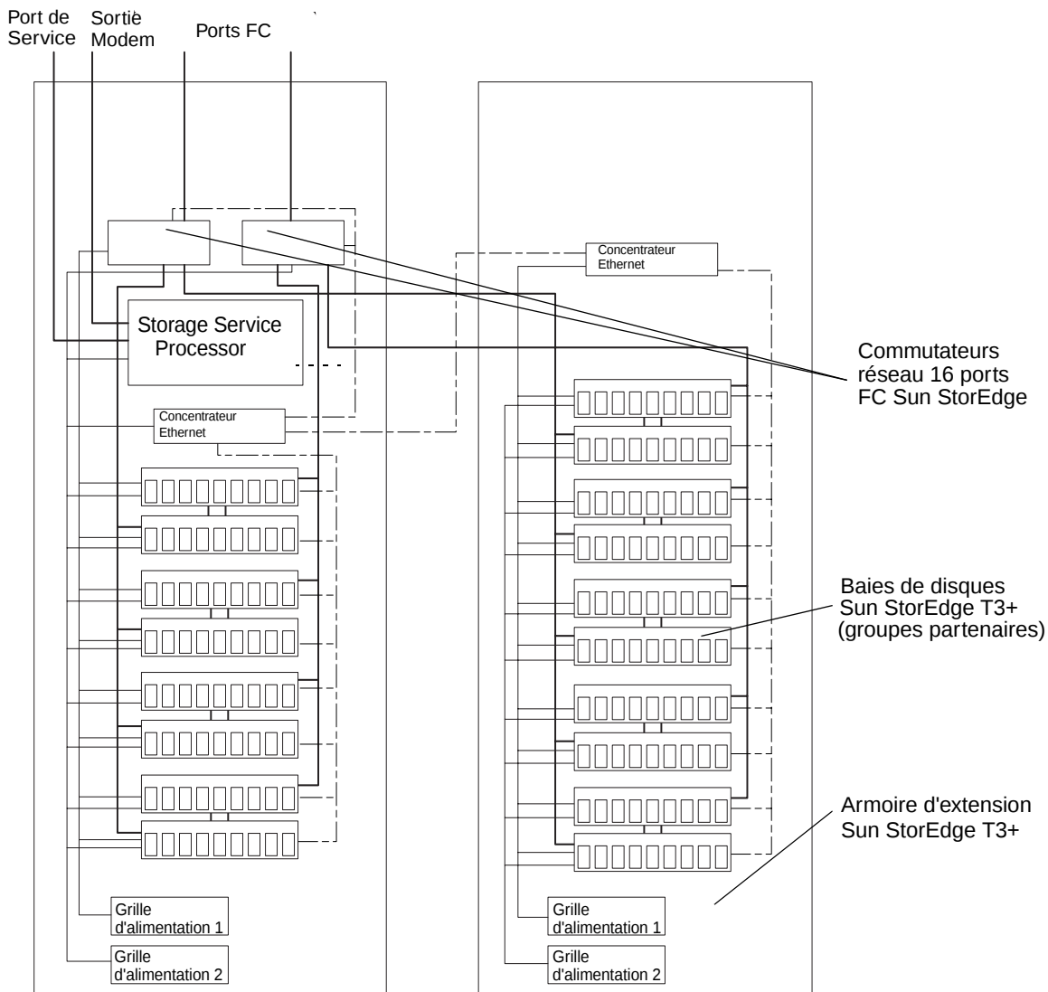
FIGURE 1-2 Système Sun StorEdge 3960
