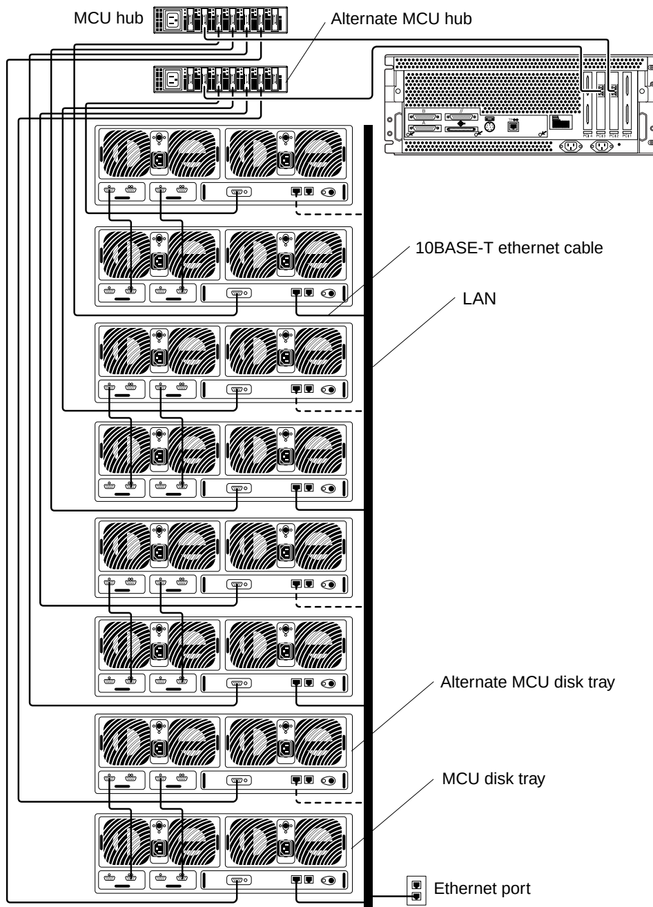
FIGURE 1 Maximum Configuration for the Sun StorEdge N8400 Filer
