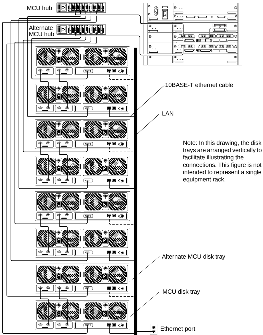
FIGURE 1 Minimum Configuration for the Sun StorEdge N8600 Filer
