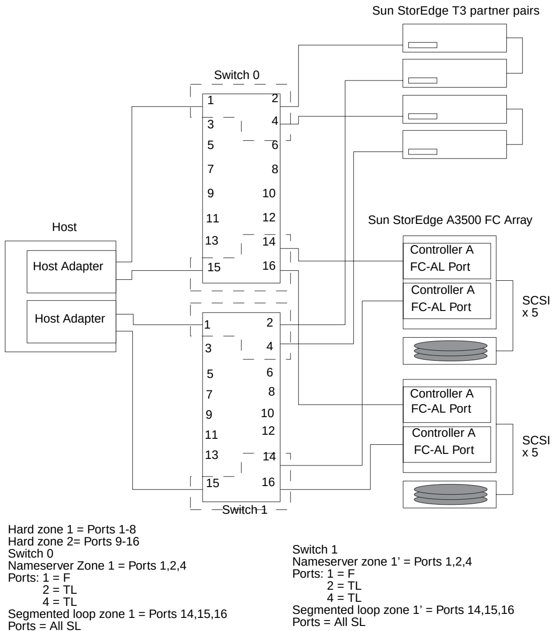
FIGURE 2-8 Single Host Connected to Multiple Sun StorEdge T3 Arrays and Multiple Sun StorEdge A3500FC Arrays
