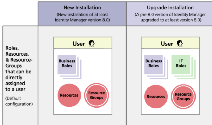
FIGURE 5-2 Roles and resources that can be directly assigned to users.
