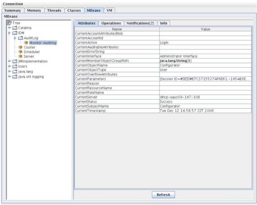
FIGURE 10-3 Viewing MBean Attributes in JConsole
