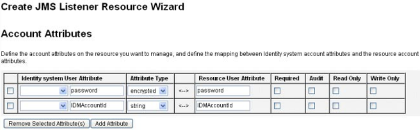
FIGURE 11-12 The Account Attributes Page of the Create JMS Listener Resource Wizard
