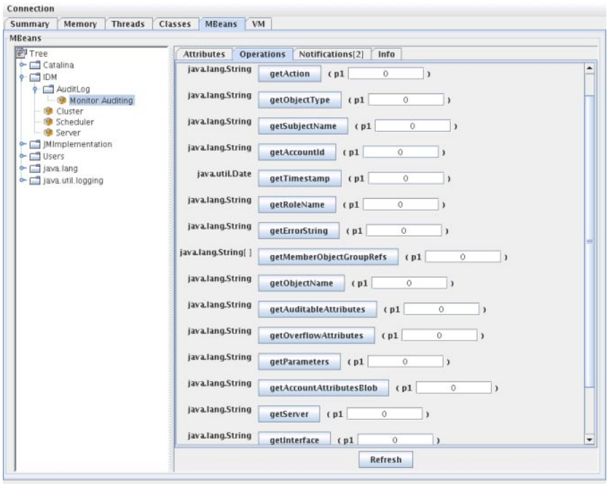
FIGURE 10-2 Querying the MBean for Additional Information in JConsole
