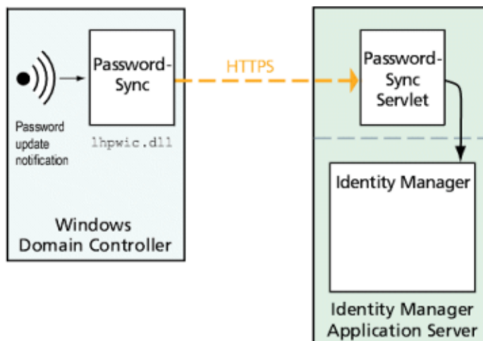
FIGURE 11-1 PasswordSync Logical Diagram (Direct Connection)
