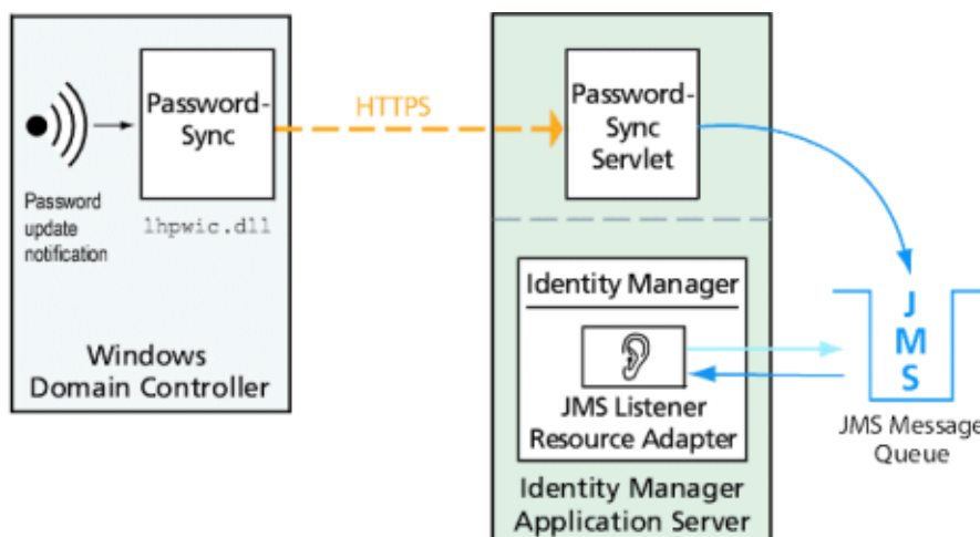
FIGURE 11-2 PasswordSync Logical Diagram (JMS Connection).
