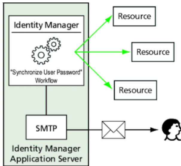
FIGURE 11–3 PasswordSync Triggers a Workflow
