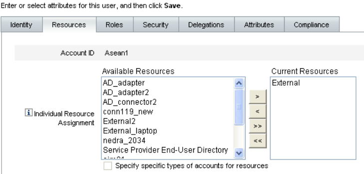
FIGURE 5-19 Edit User Page
