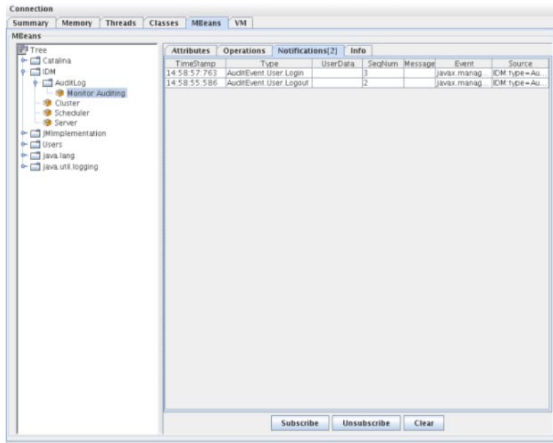
FIGURE 10-1 Viewing JMX Audit Event Notifications in JConsole
