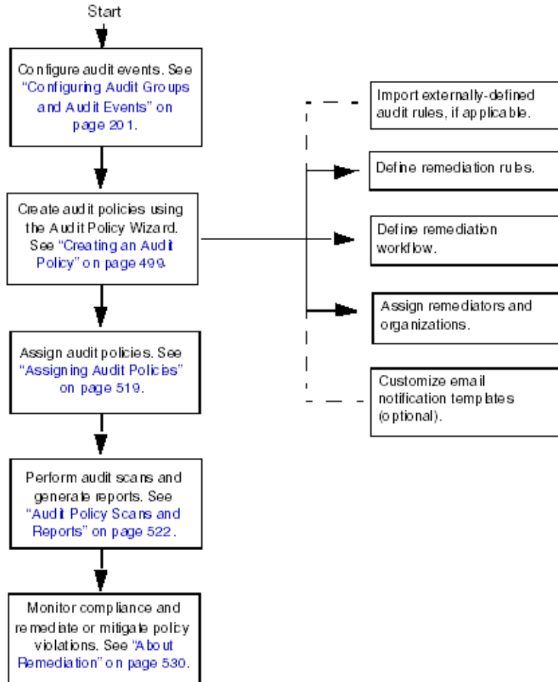
FIGURE 13-1 A Logical Task Flow for Establishing Policy-based Compliance
