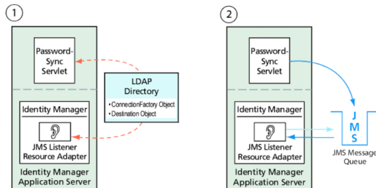
FIGURE 11–14 Retrieving Connection Factory and Destination Objects from the LDAP Directory
