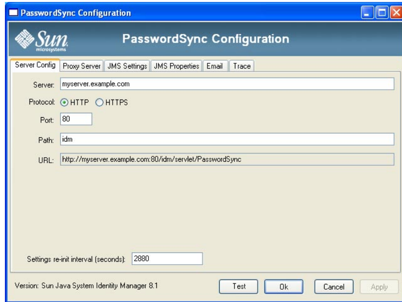
FIGURE 11-4 PasswordSync Configuration Wizard
