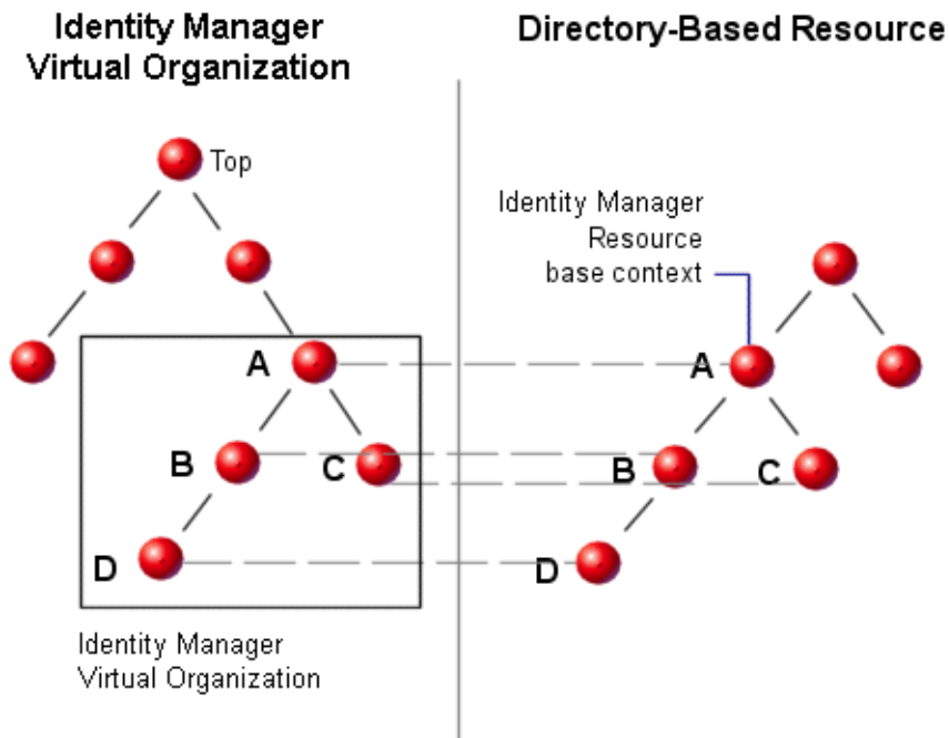
FIGURE 6-2 Identity Manager Virtual Organization
