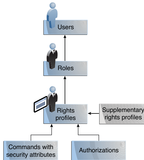
FIGURE 8-1 Solaris RBAC Element Relationships
