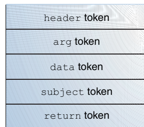
FIGURE 31-3 Typical Audit Record Structure
