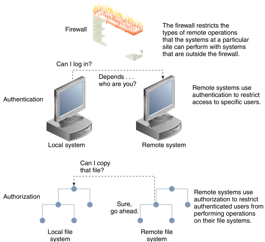
FIGURE 2-1 Security Restrictions for Remote Operations
