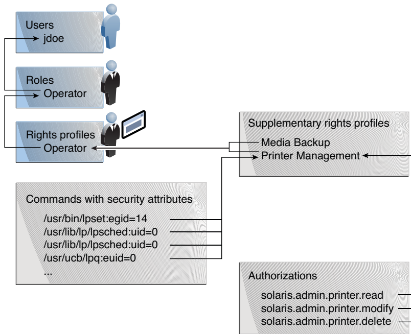
FIGURE 8-2 Example of Solaris RBAC Element Relationships
