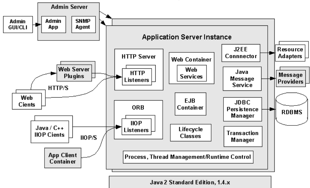
Figure 1-1 Sun ONE Application Server deployment
