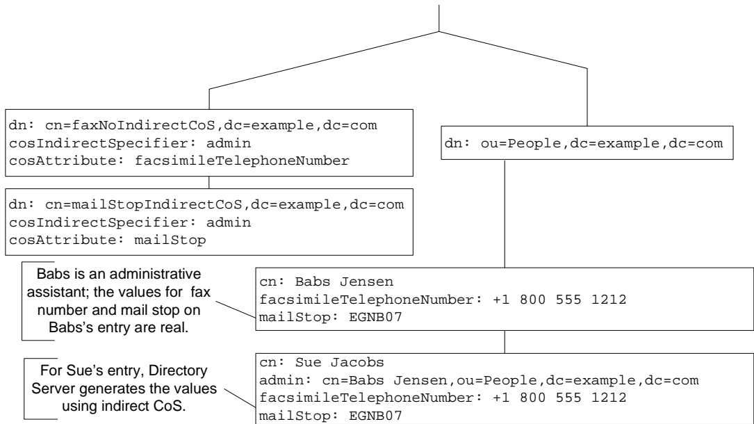
Figure 7-6 Generating Mail Stop and Fax Number With Indirect CoS
