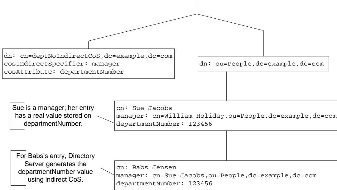
Figure 7-5 Generating DepartmentNumber With Indirect CoS
