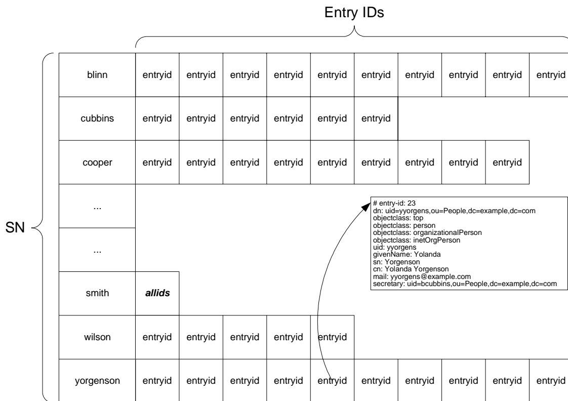
Figure 4-2 Representation of an Equality Index
