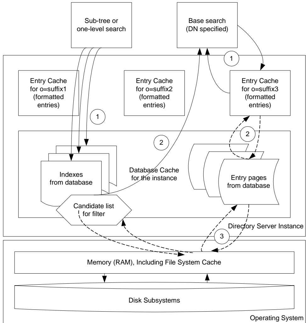
Figure 3-2 Searches and Cache
