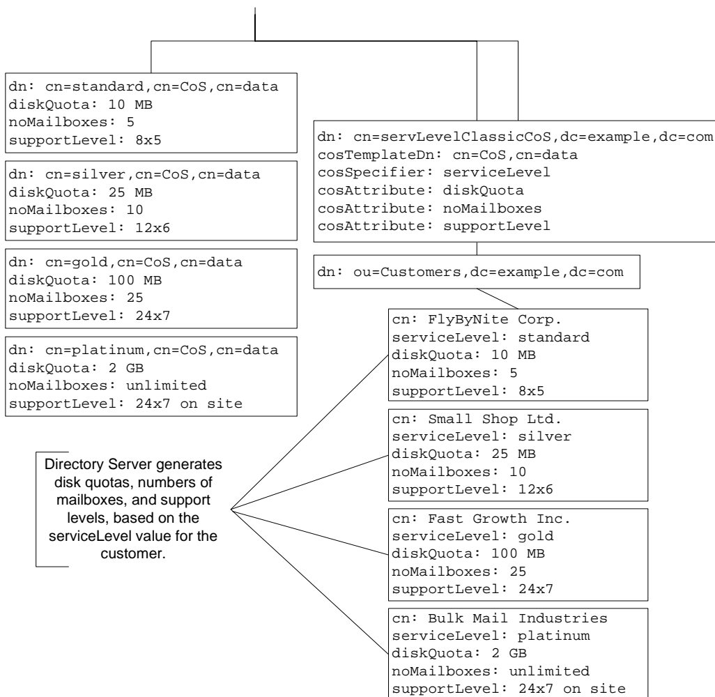
Figure 7-7 Generating Service Level Data With Classic CoS
