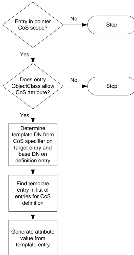
Figure 7-3 Classic CoS Operation
