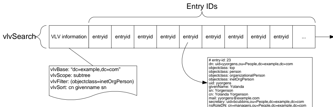
Figure 4-4 Representation of a Browsing Index
