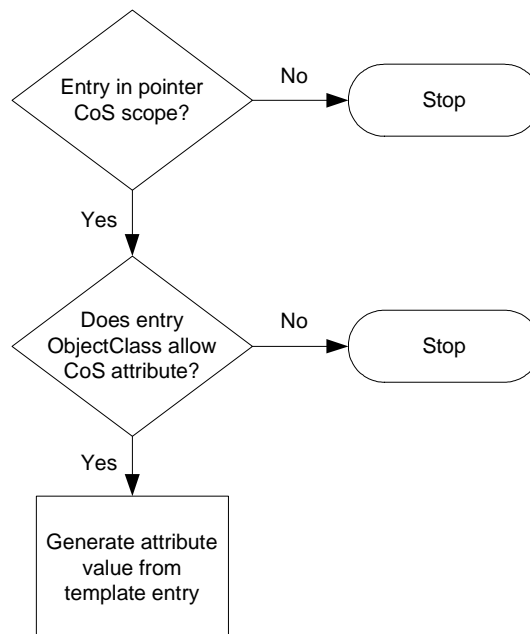
Figure 7-1 Pointer CoS Operation
