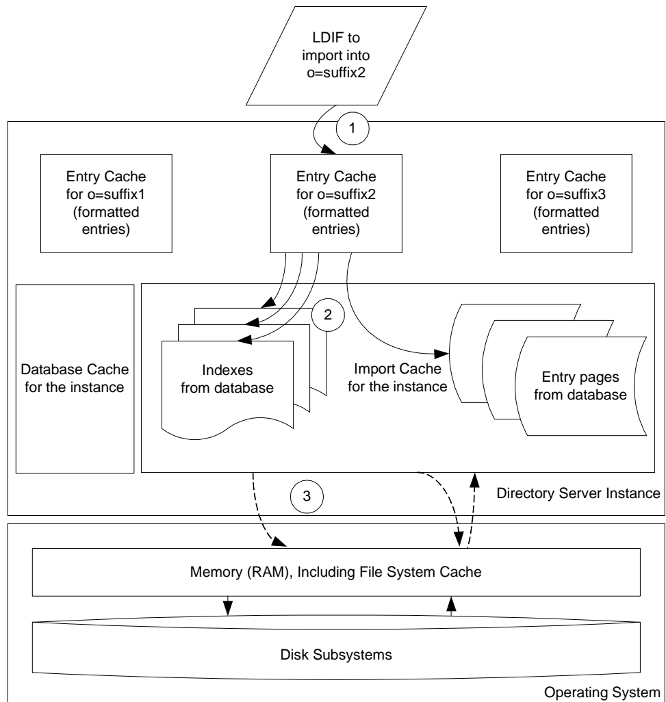
Figure 3-4 Suffix Initialization (Bulk Loading) and Cache
