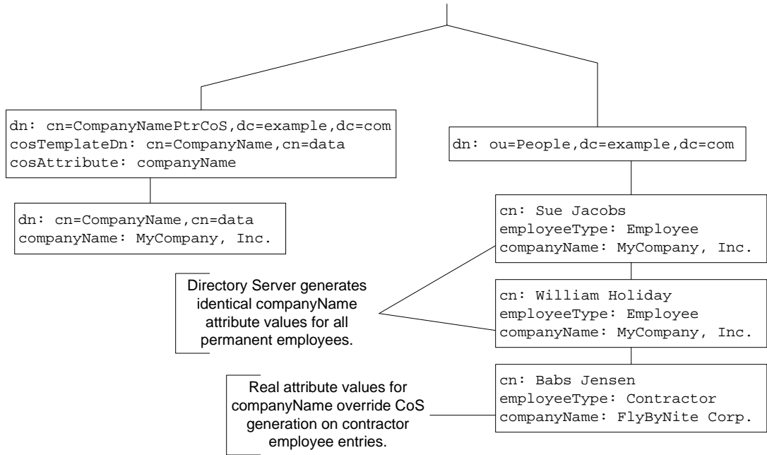
Figure 7-4 Generating CompanyName With Pointer CoS
