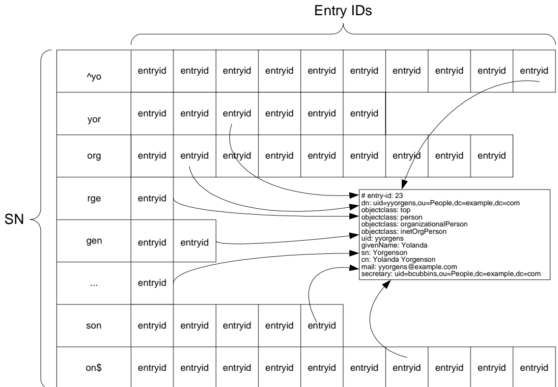
Figure 4-3 Representation of a Substring Index
