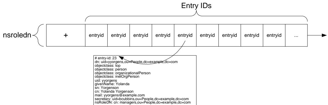
Figure 4-1 Representation of a Presence Index
