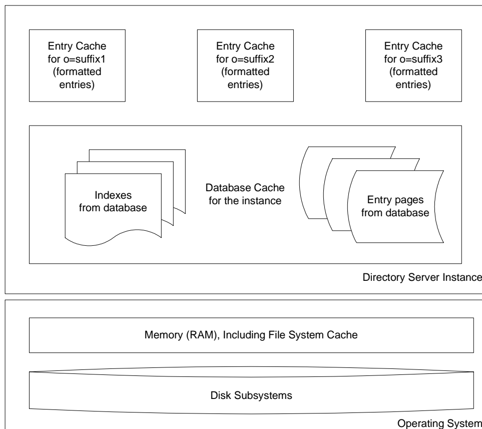
Figure 3-1 Entry and Database Caches in Context
