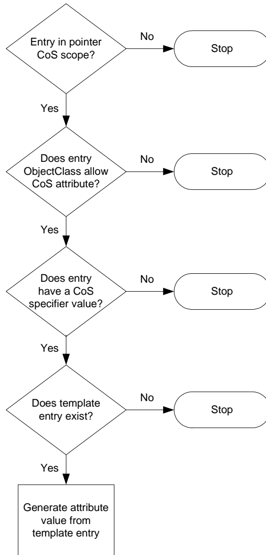
Figure 7-2 Indirect CoS Operation
