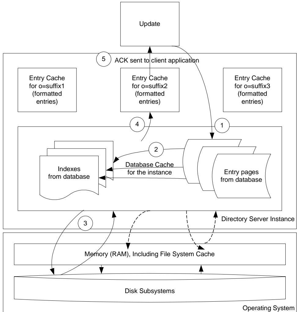
Figure 3-3 Updates and Cache
