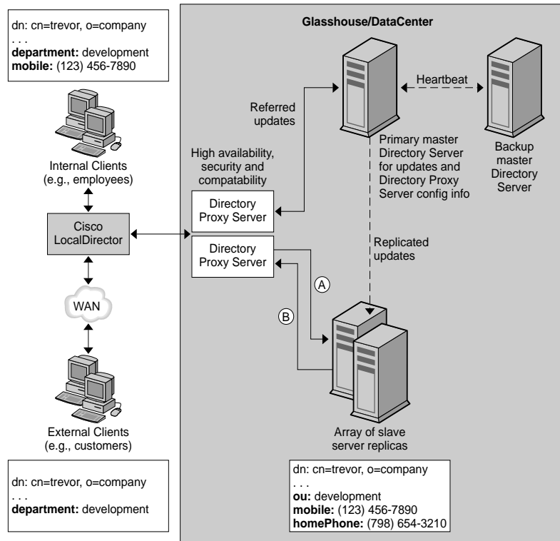
Figure 2-3 A Centralized LDAP Directory Infrastructure
