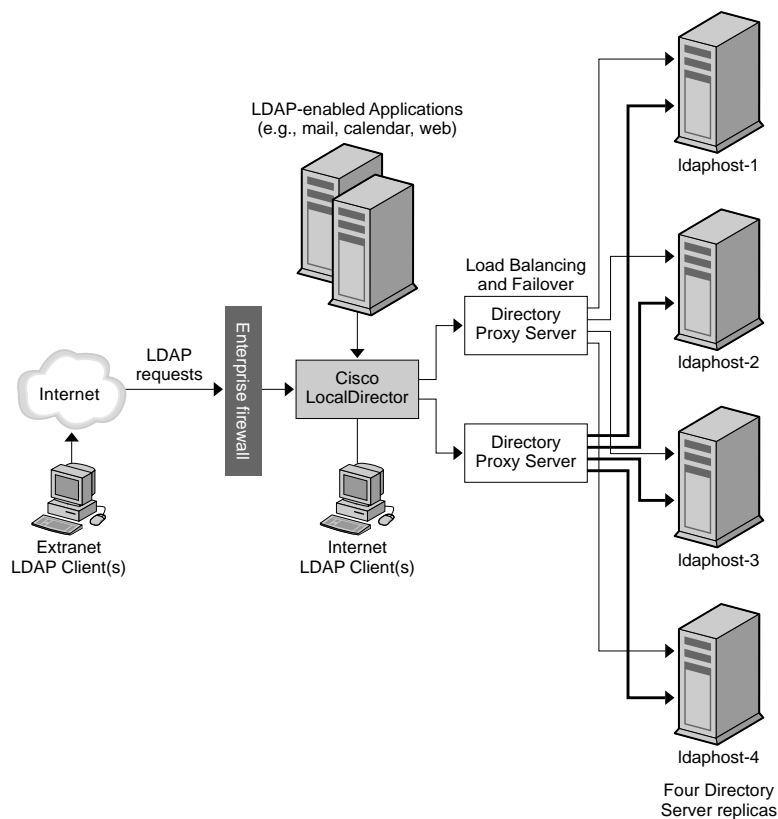
Figure 2-1 Internal High Availability Configuration
