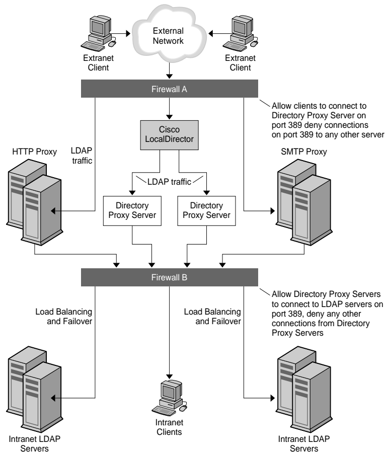
Figure 2-5 Directory Proxy Server Setup With Two Firewalls
