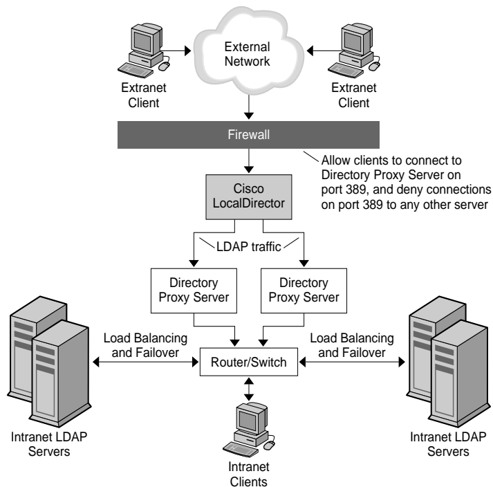
Figure 2-4 Directory Proxy Server Setup With One Firewall
