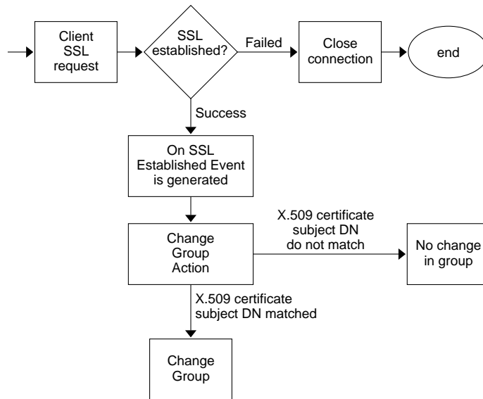
Figure 12-2 Certificate-Based Authentication of Clients
