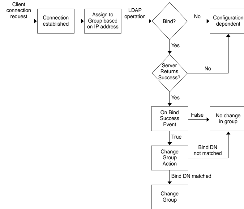
Figure 7-2 Directory Proxy Server Decision Tree for Determining Group Membership
