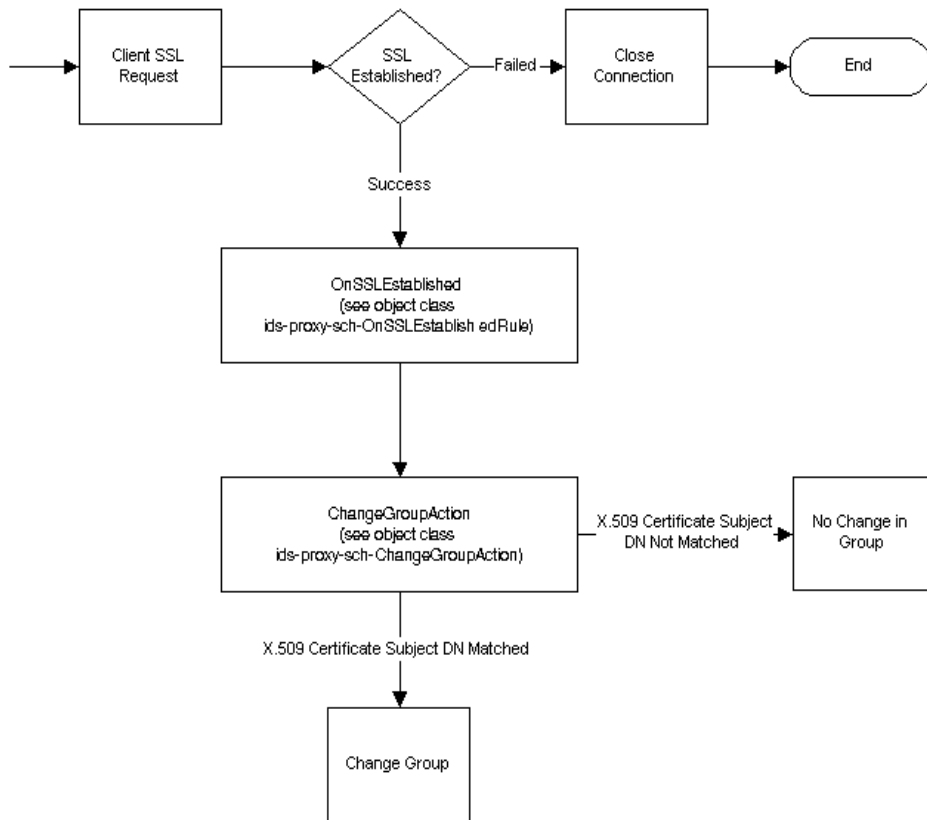
Figure A-2 Change Group on Establishment of TLS
