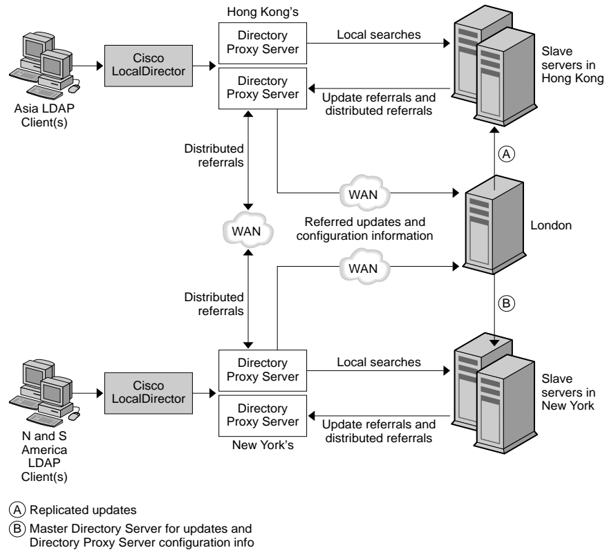
Figure 2-2 A Distributed LDAP Directory Infrastructure
