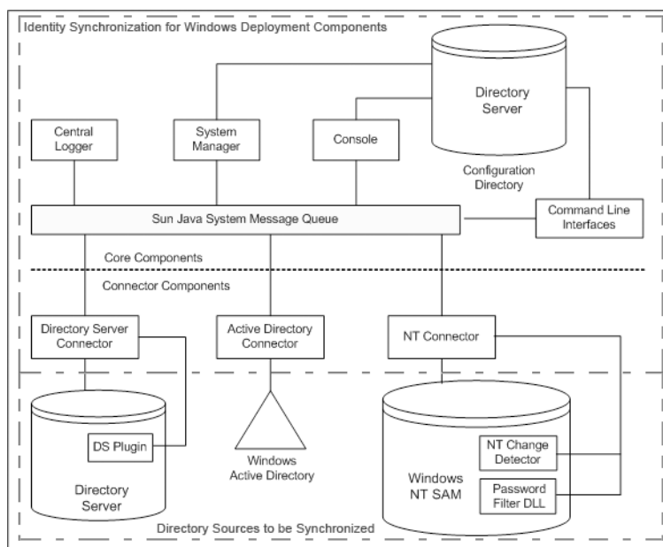
FIGURE 3-1 System Components
