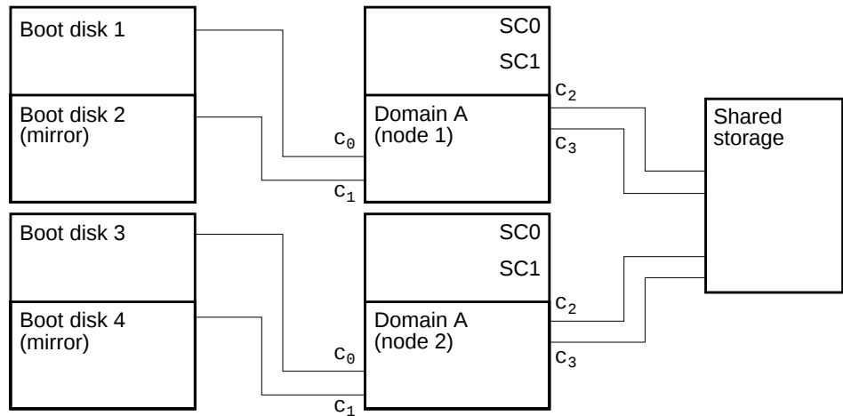
FIGURE 2-3 Storage Connections
