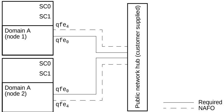
FIGURE 1-2 Public Network
