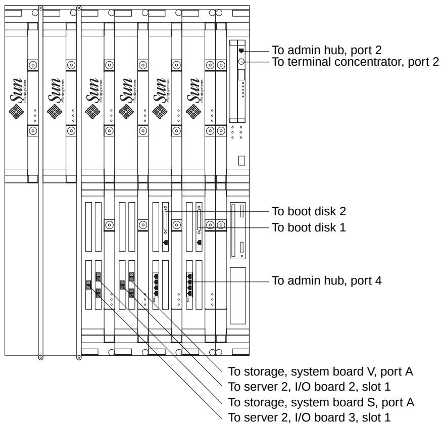
FIGURE 2-5 Server 1 Front Cable Connections
