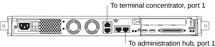
FIGURE B-1 Management Server Cable Connections
