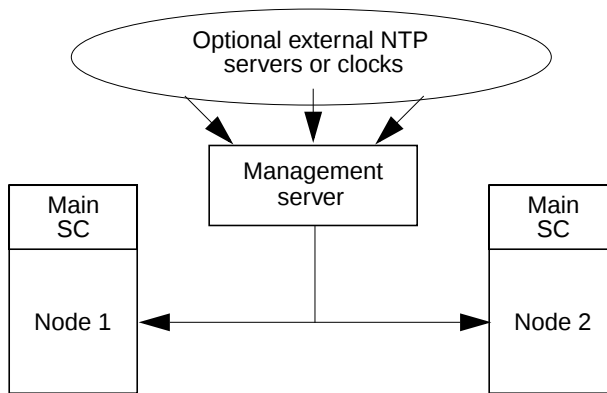
FIGURE 1-7 NTP Architecture
