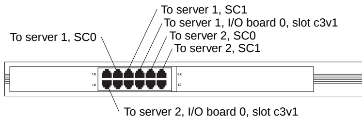
FIGURE 2-12 Administration Hub Cable Connections
