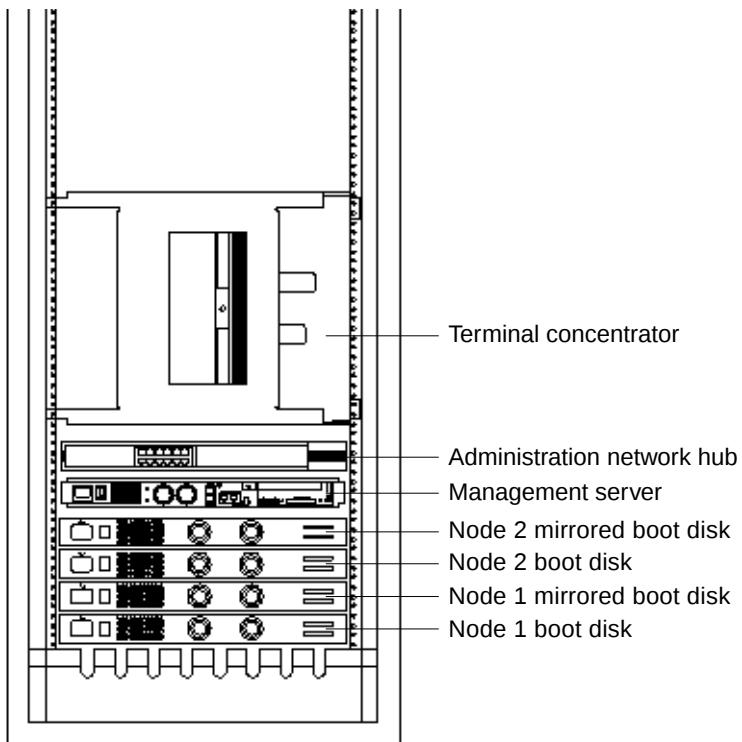
FIGURE 2-2 Expansion Cabinet Component Placement
