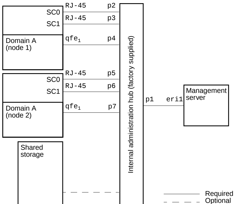
FIGURE 1-3 Internal Administration Network
