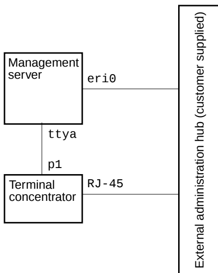
FIGURE 1-4 External Administration Network
