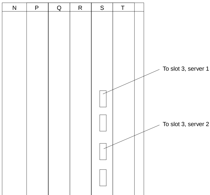
FIGURE 2-9 Storage Cabinet System Board S Connections
