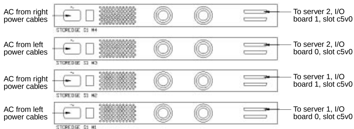
FIGURE 2-13 Boot Disks Cable Connections
