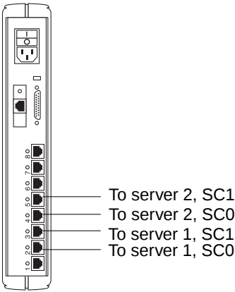
FIGURE 2-11 Terminal Concentrator Cable Connections
