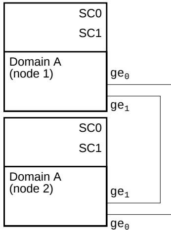
FIGURE 1-1 Private Interconnect
