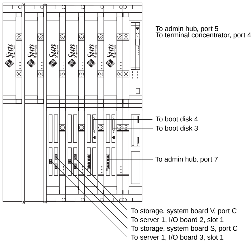
FIGURE 2-7 Server 2 Front Cable Connections
