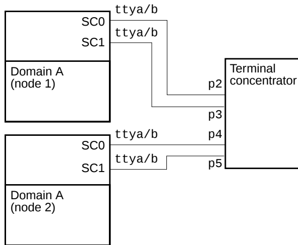
FIGURE 2-4 Serial Connections
