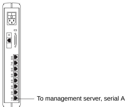
FIGURE B-2 Terminal Concentrator Cable Connections
