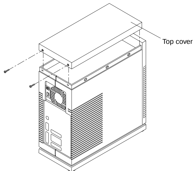
Figure 5-10 Removing and Replacing the Top Cover to the Tower Unit
