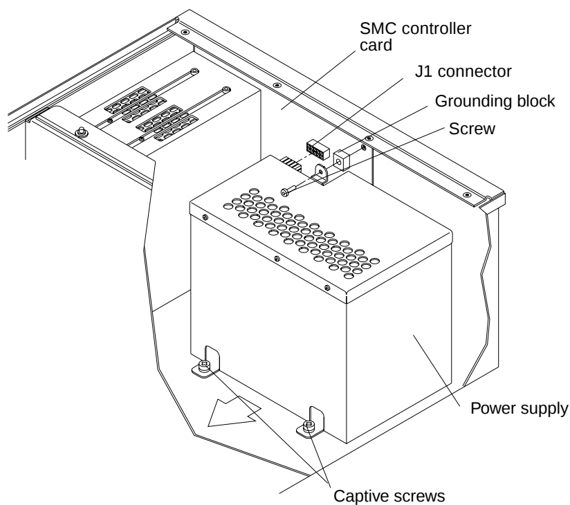
Figure 6-6 Removing the Screws Inside the Chassis from the Power Supply
