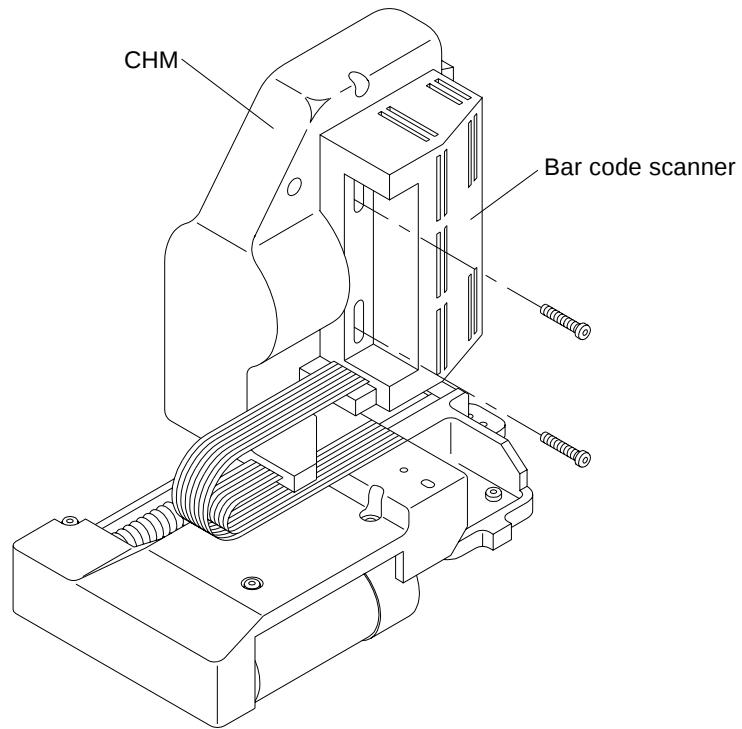
Figure 6-24 Attaching the Bar Code Scanner
