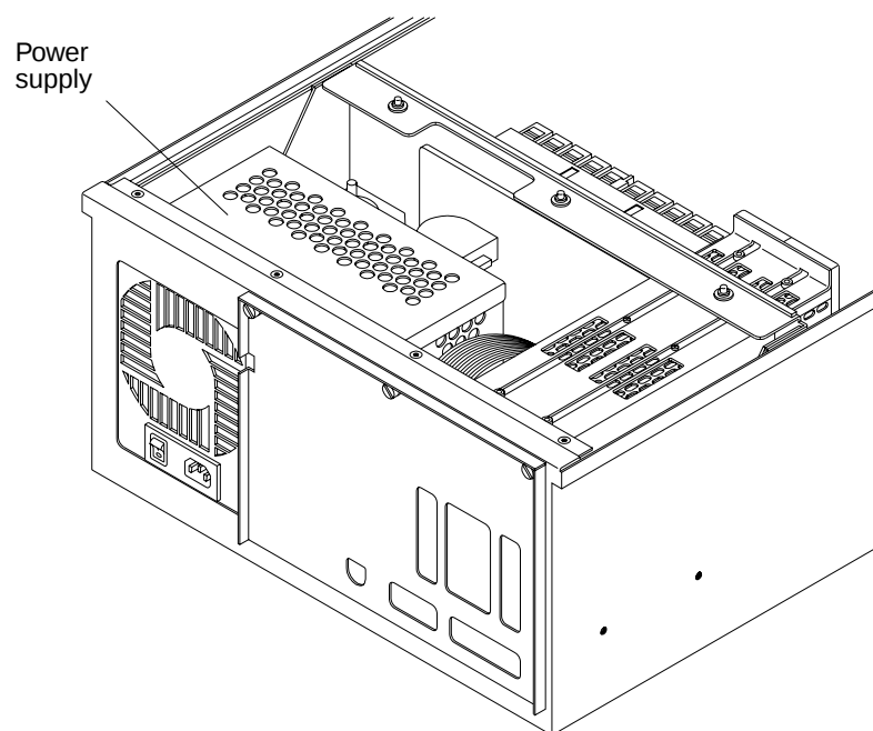
Figure 7-5 Location of the Power Supply
