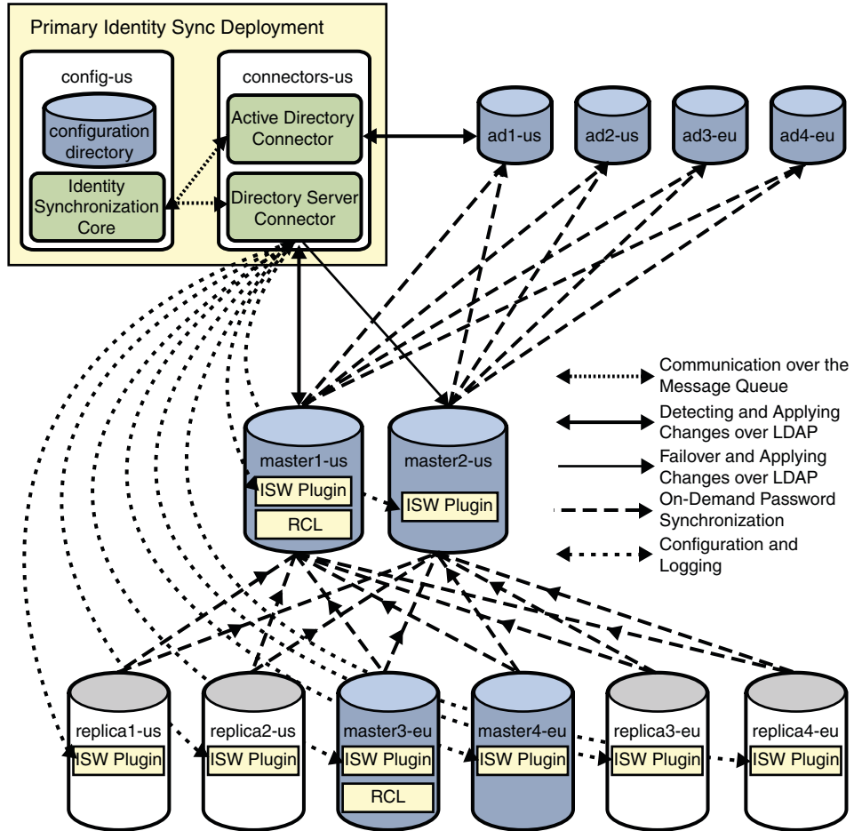
FIGURE 3-5 Primary Installation after Reinstalling the Identity Synchronization for Windows Plugins
