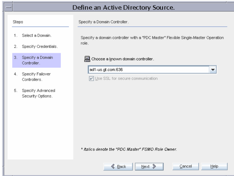
FIGURE 3-9 Configuring the Active Directory Domain
