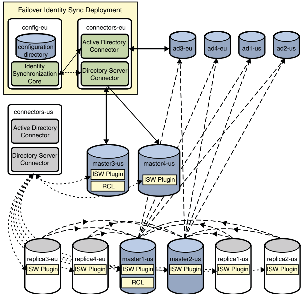
FIGURE 3-4 Failover Installation while the Primary Installation is Active
