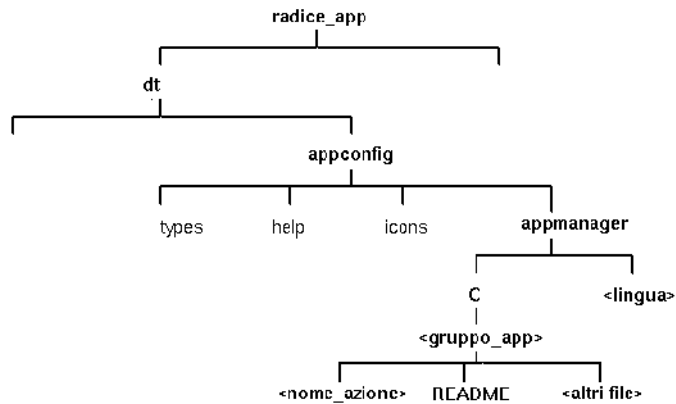
FIGURA 5-7 La directory appmanager
