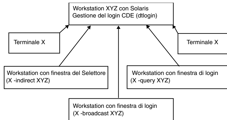
FIGURA 6-1 Desktop in rete
