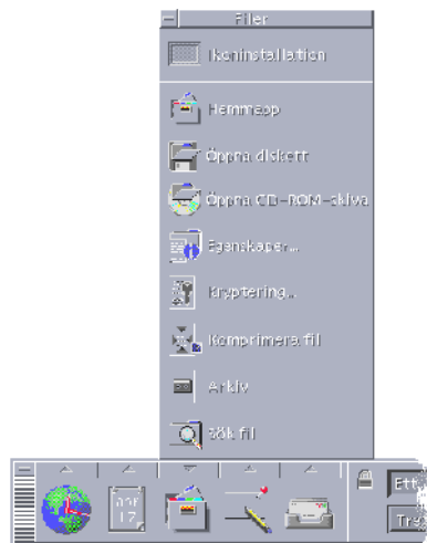
FIGUR 1-3 Filer, panelundermeny
