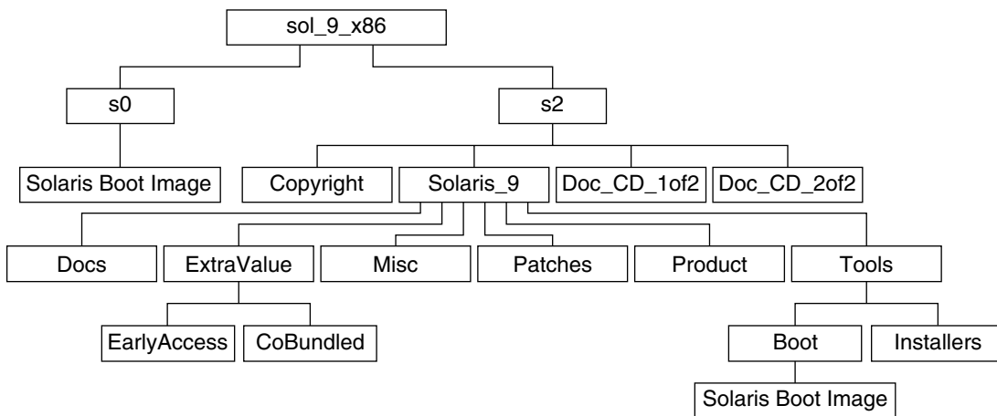
FIGUR B-6 Solaris-dvd (x86-version)
