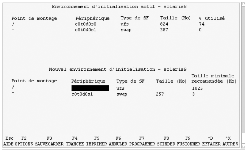
FIGURE 35-3 Menu Configuration de Solaris Live Upgrade
