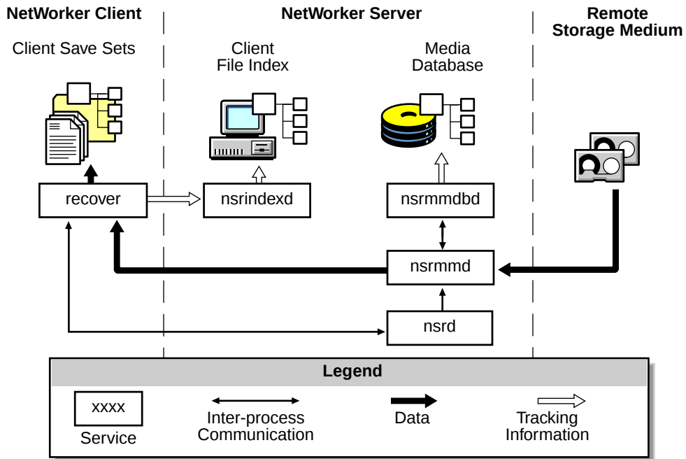
Figure 2. Processes and Programs During a Recover Session
