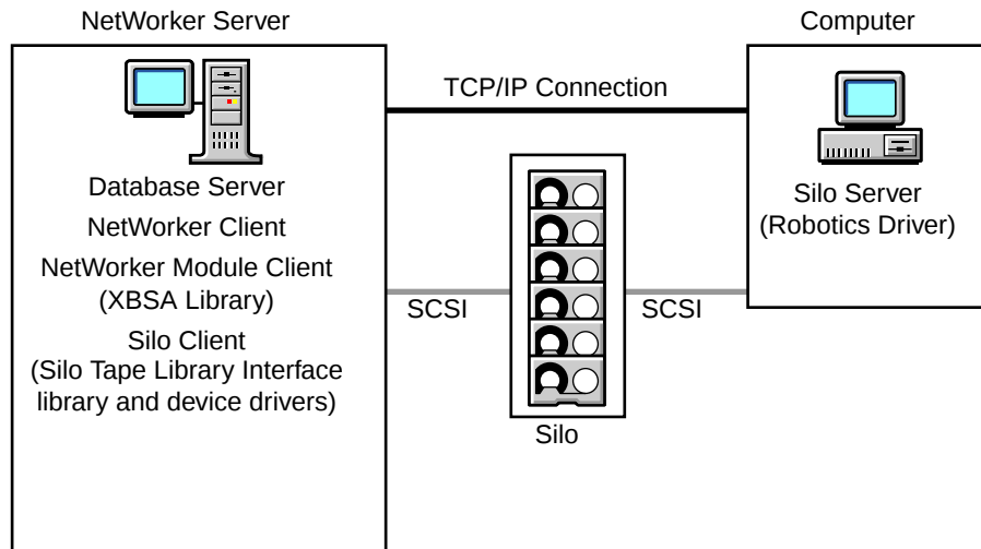
Figure 6. Local Backup to a Silo
